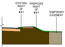
PROPOSED ROADWAY SECTION - MILLPOND RD EASTBOUND RIGHT OF WAY AND TEMPORARY EASEMENTS REQUIRED
