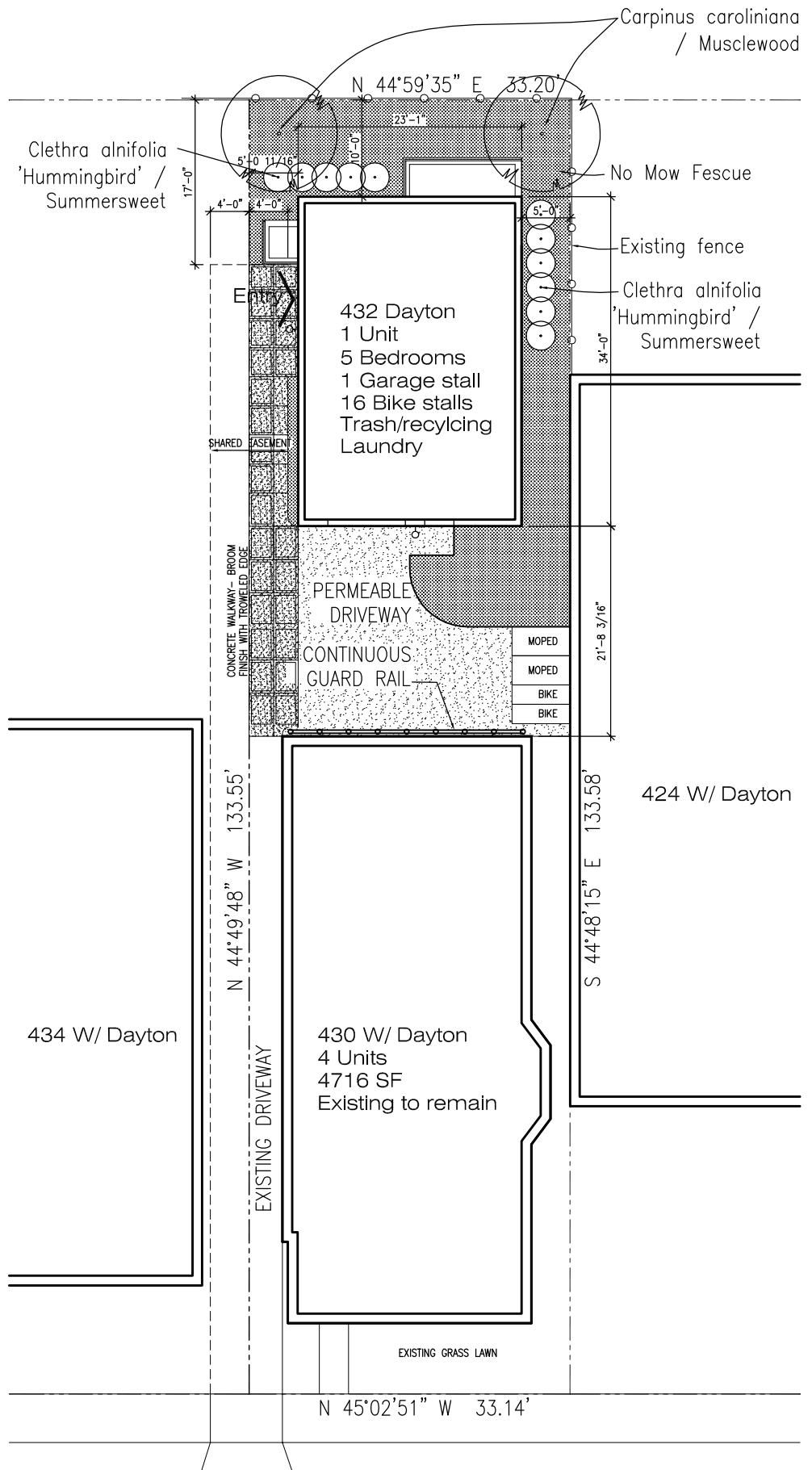
Site Plan 1/16" = 1'-0"
