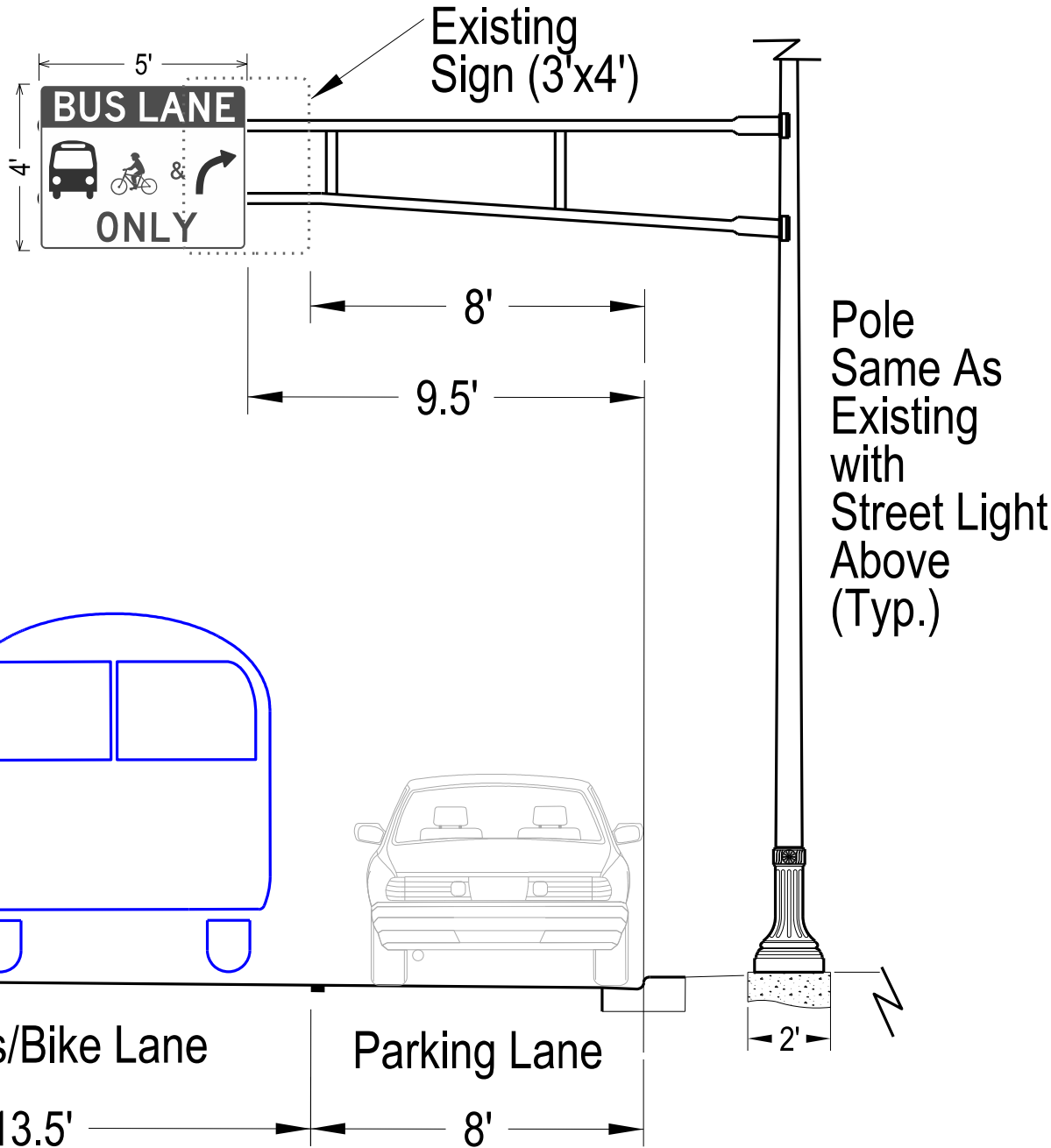
Bus/Bike Lane Overhead Sign Placement
