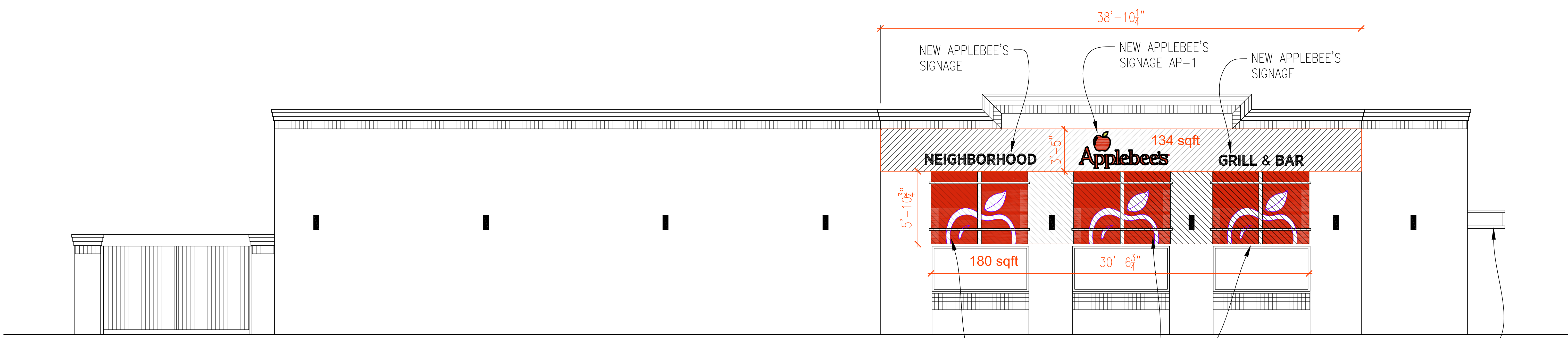
PROPOSED SOUTH EXTERIOR ELEVATION SCALE - 1/4" = 1'-0"
