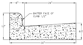
CURB AND GUTTER CROSS SECTION
