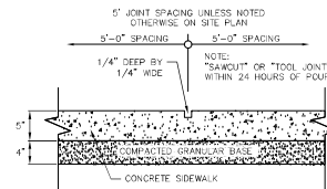
SIDEWALK CONTROL JOINT
