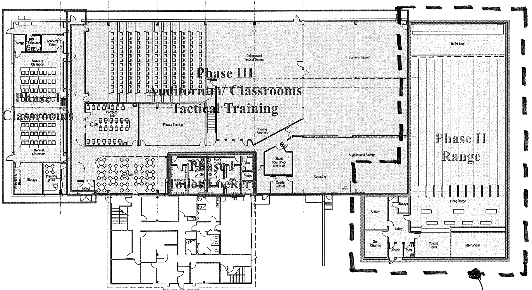
NORTH FIRST FLOOR PLAN SCALE: 1"=20'-0" (Printed at 11" x 17")
