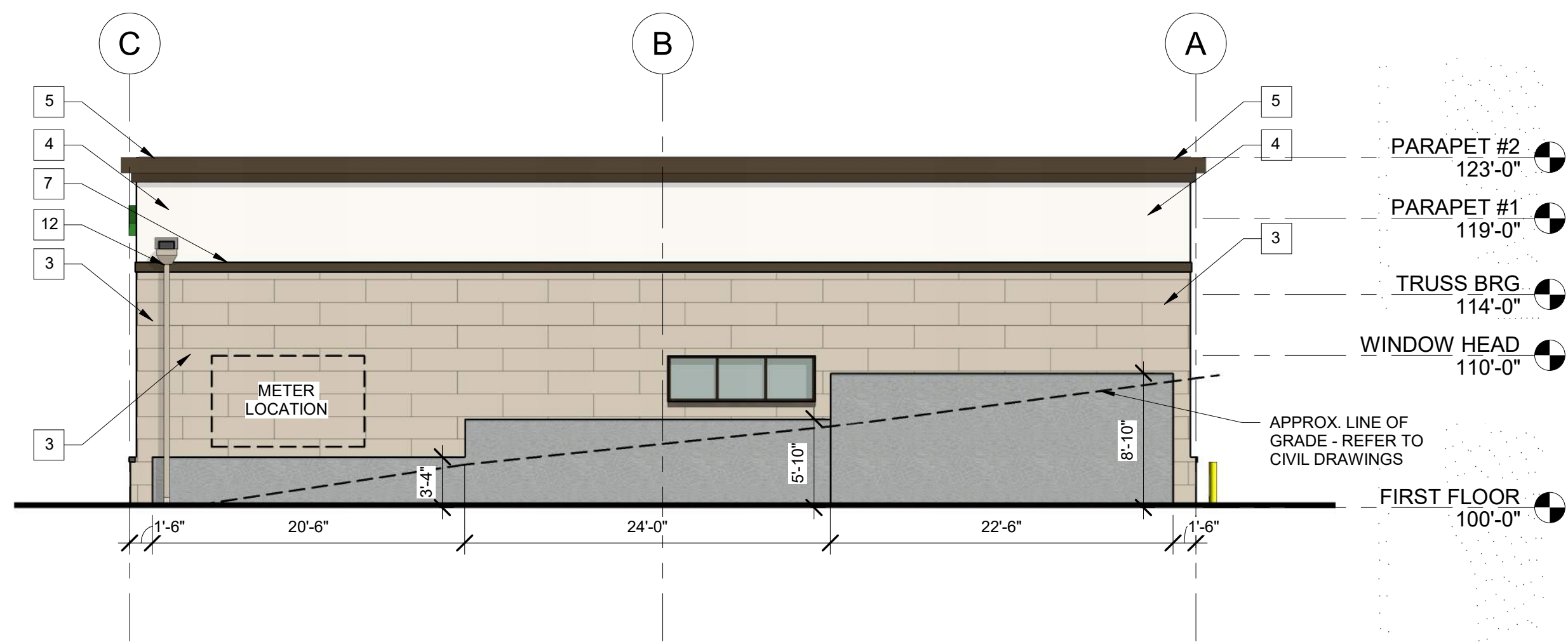
2 EAST ELEVATION 1/8" = 1'-0"
