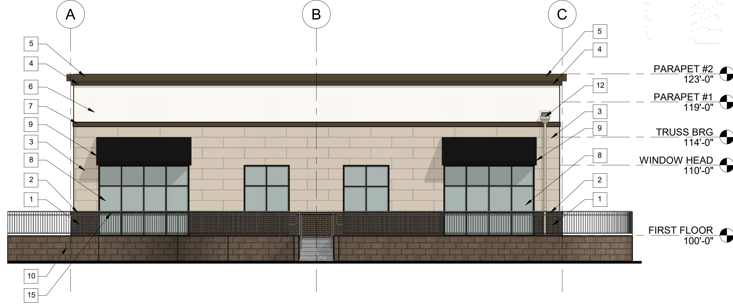
4 WEST ELEVATION 1/8" = 1'-0"
