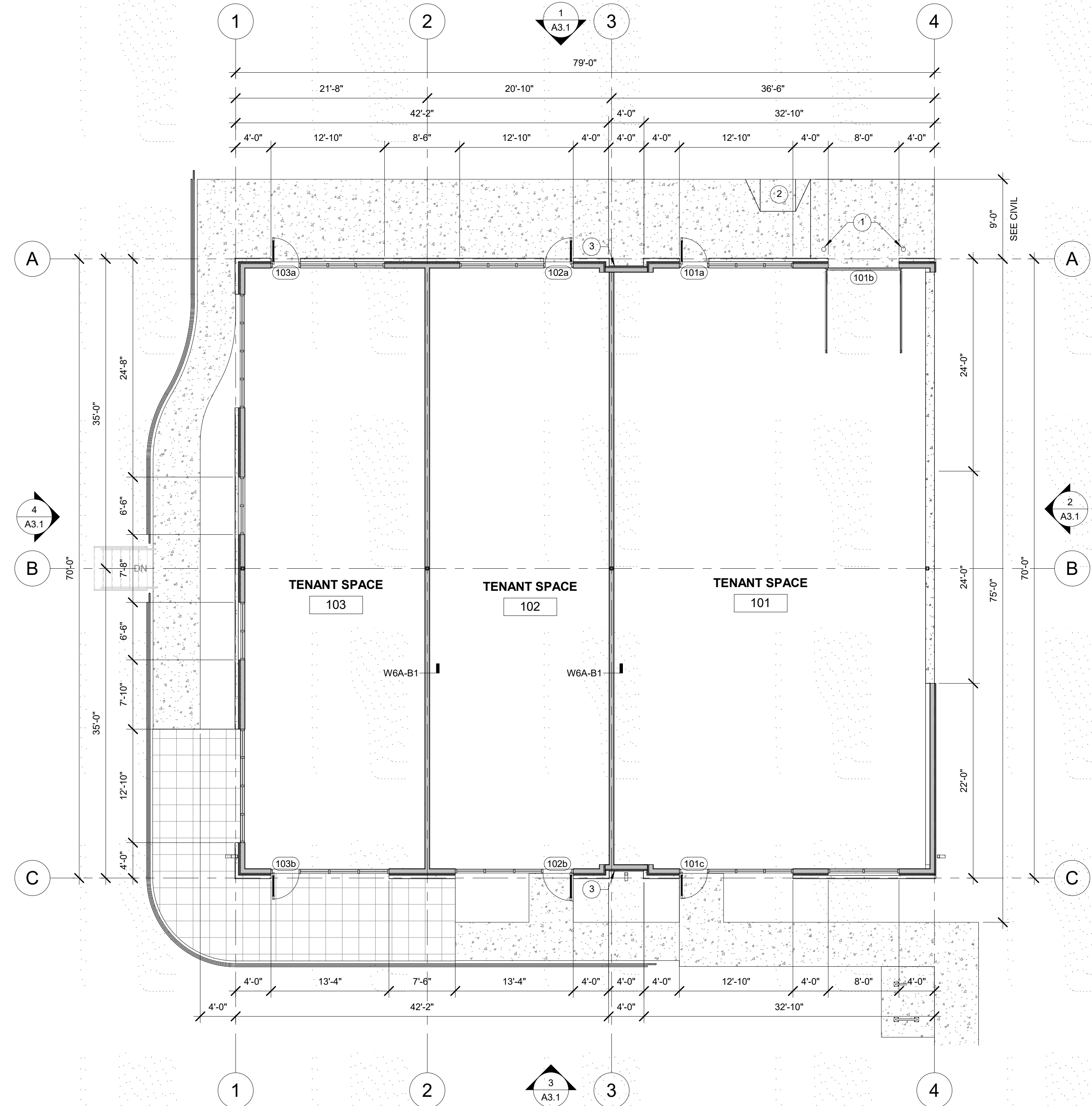
1 FLOOR PLAN 1/8" = 1'-0"
