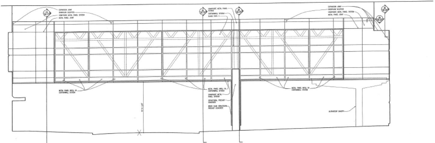
34 SOUTH ELEVATION
