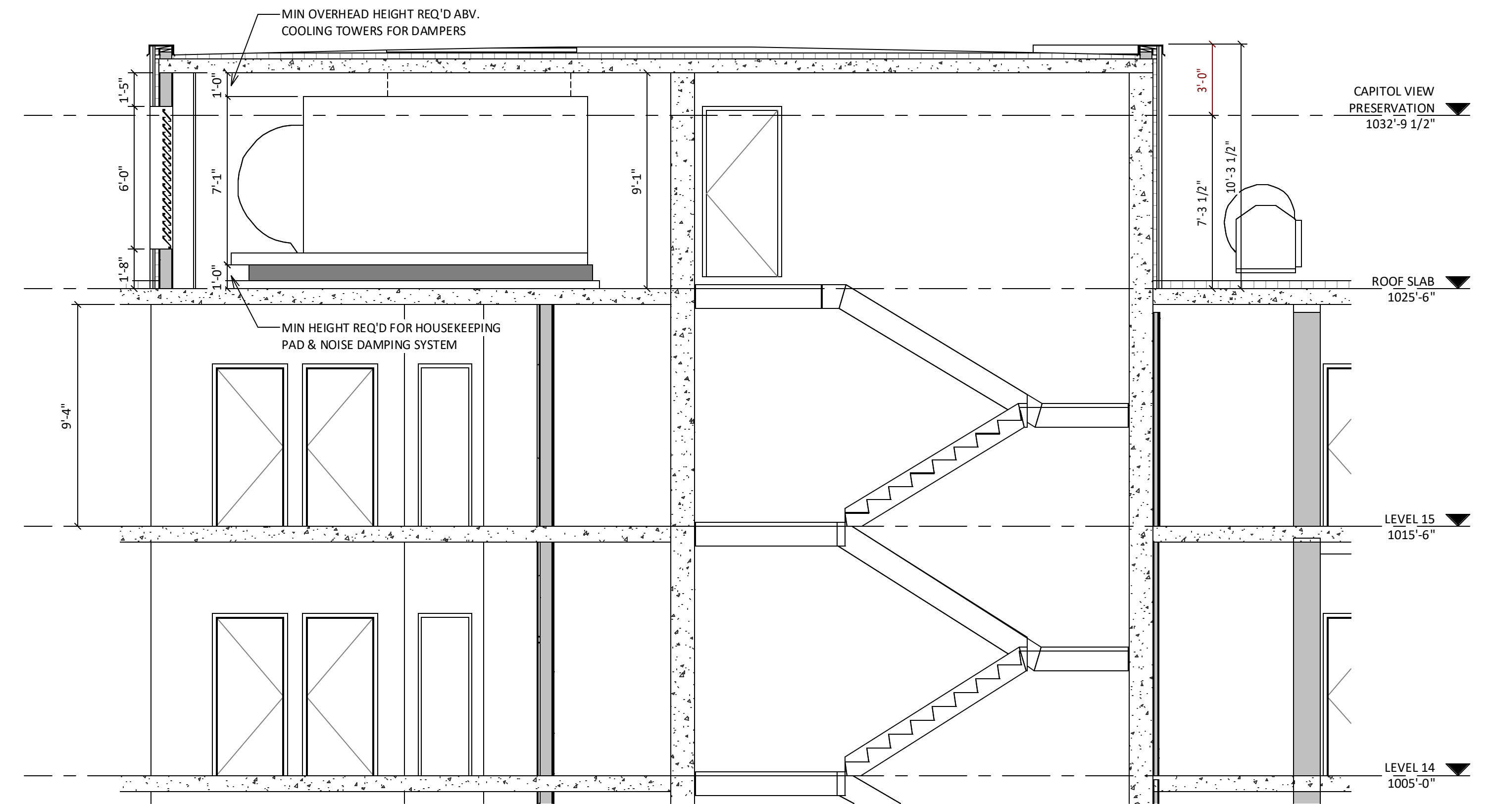
2 PENTHOUSE ROOF ACCESS 1/4" = 1'-0"
