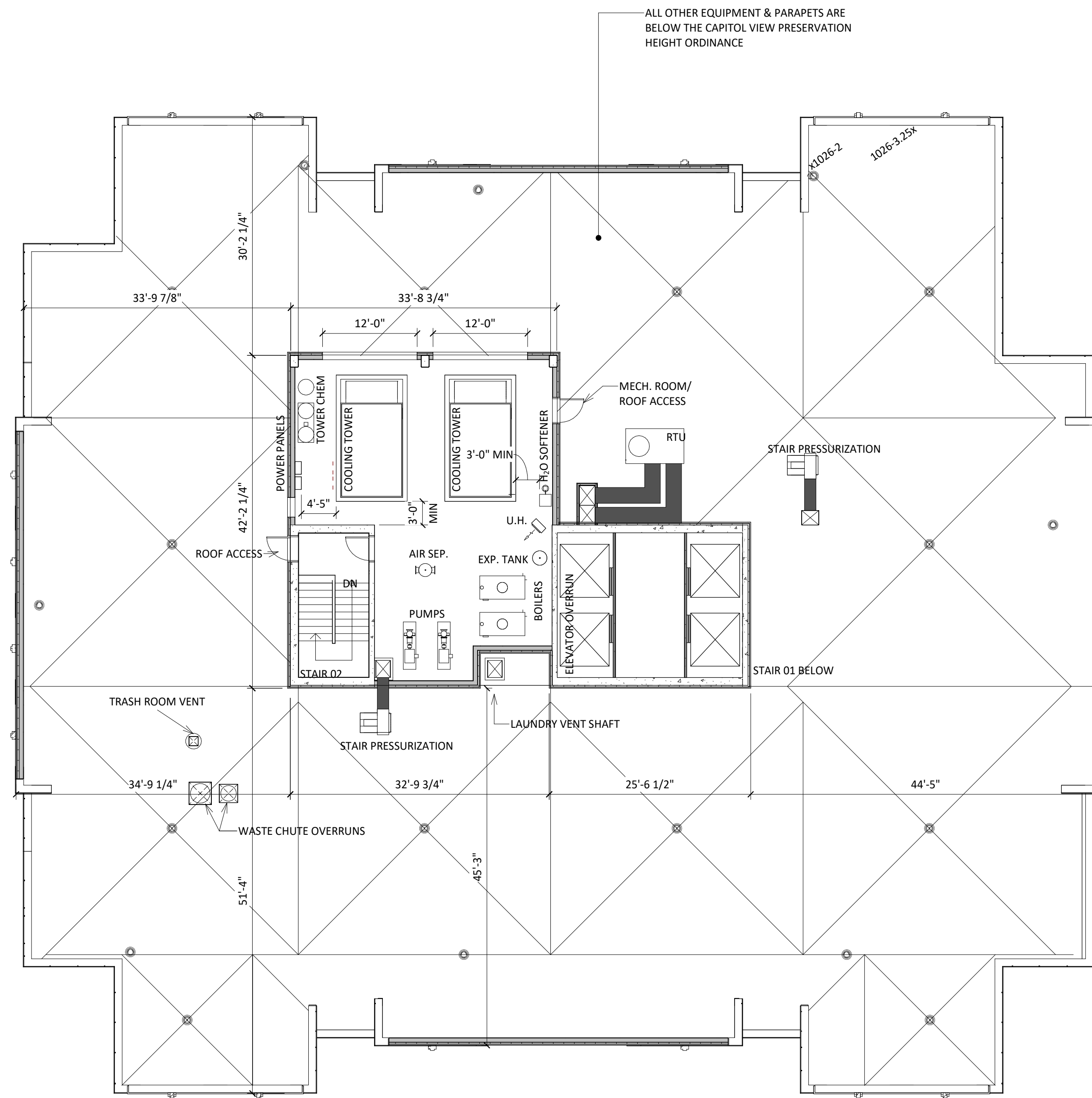
1 MECHANICAL PENTHOUSE 3/32" = 1'-0"
