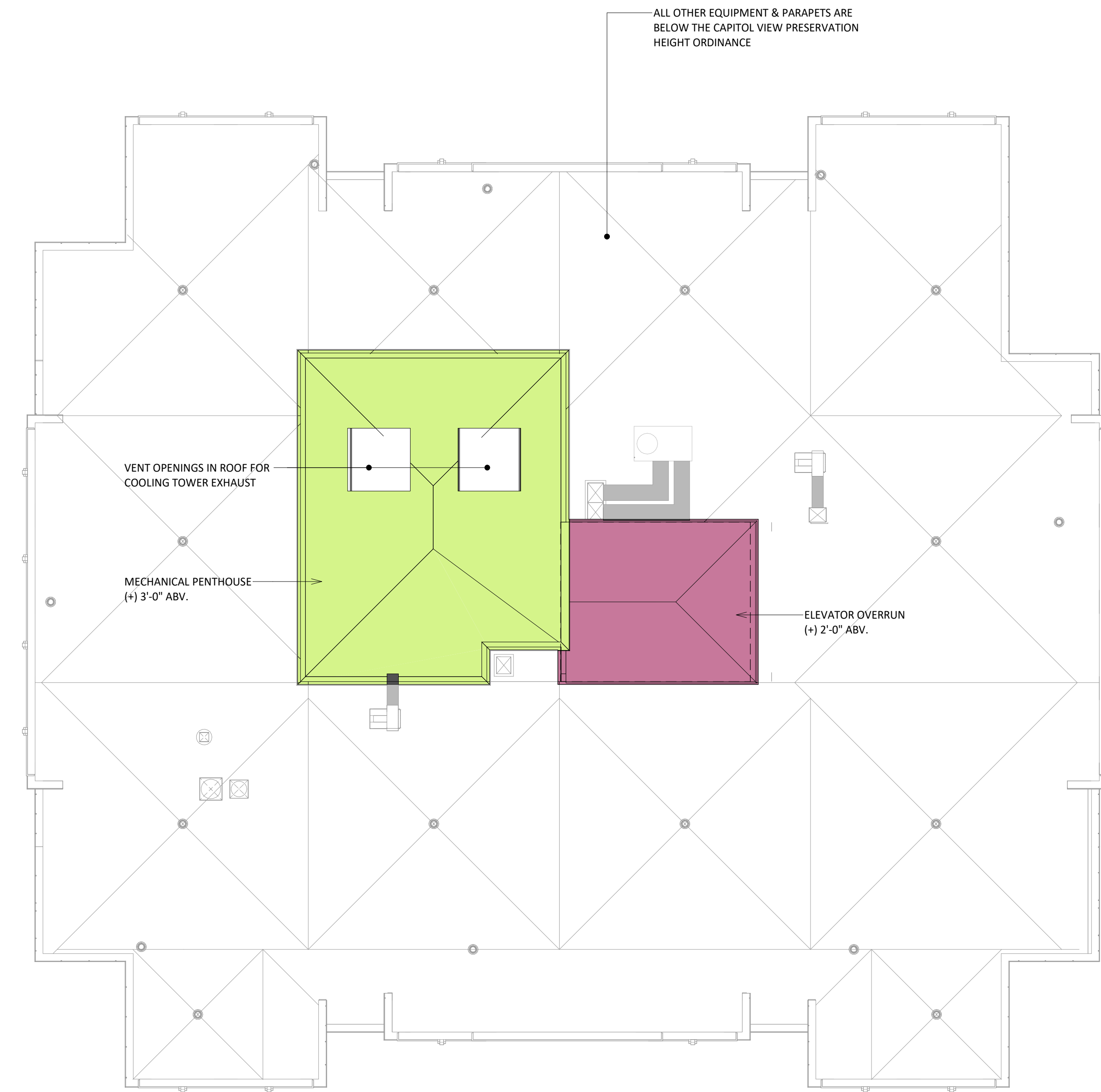
2 ROOF PLAN 3/32" = 1'-0"
