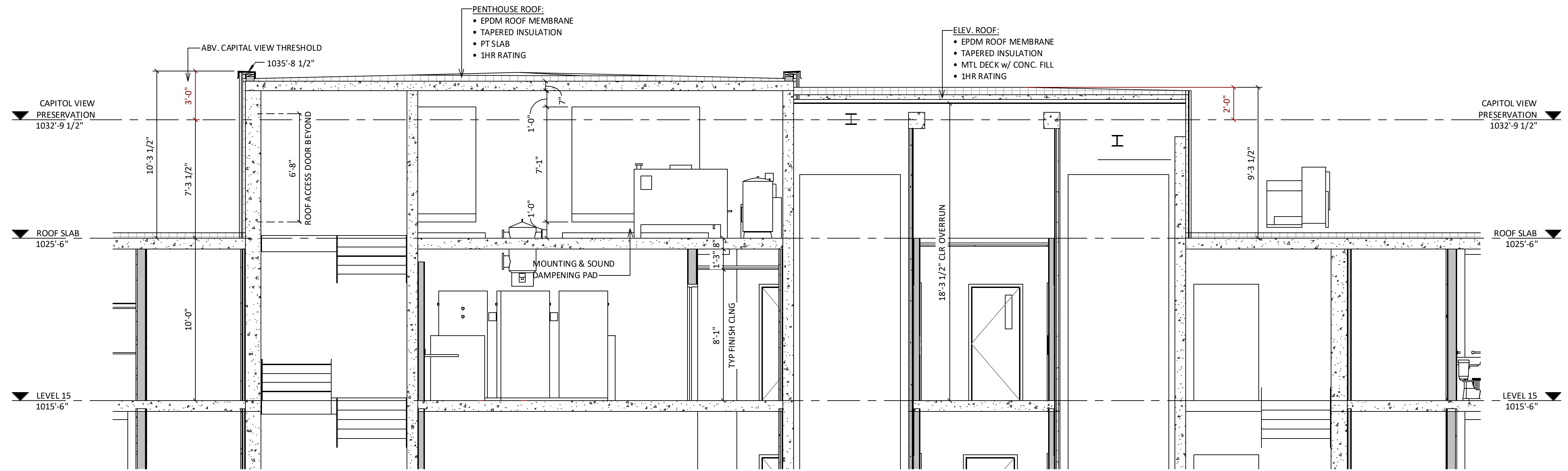
1 PENTHOUSE E/W 1/4" = 1'-0"
