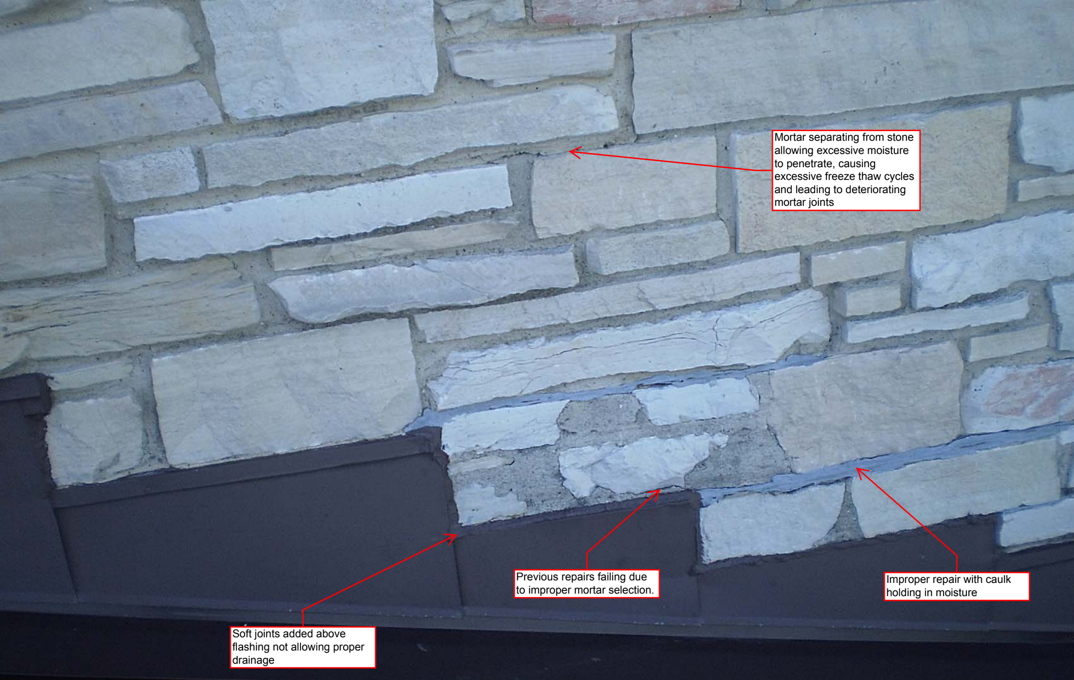
Garner Park Masonry Repairs- 2013 Typical Condition of Masonry Mortar Joints in Designated Repair Areas
