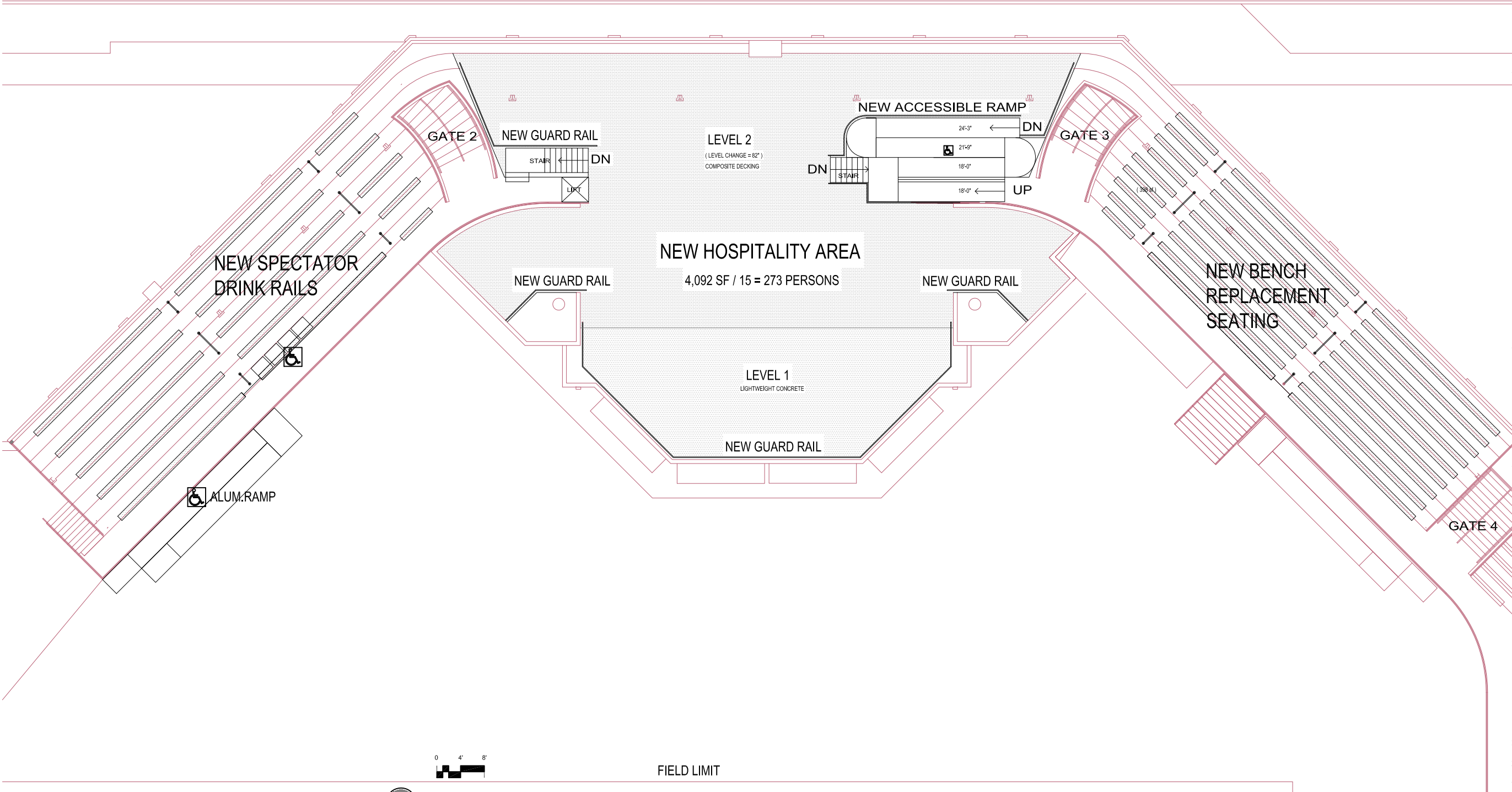
1 FLOOR PLAN - HOSPITALITY LEVEL 1/8"=1'-0"
