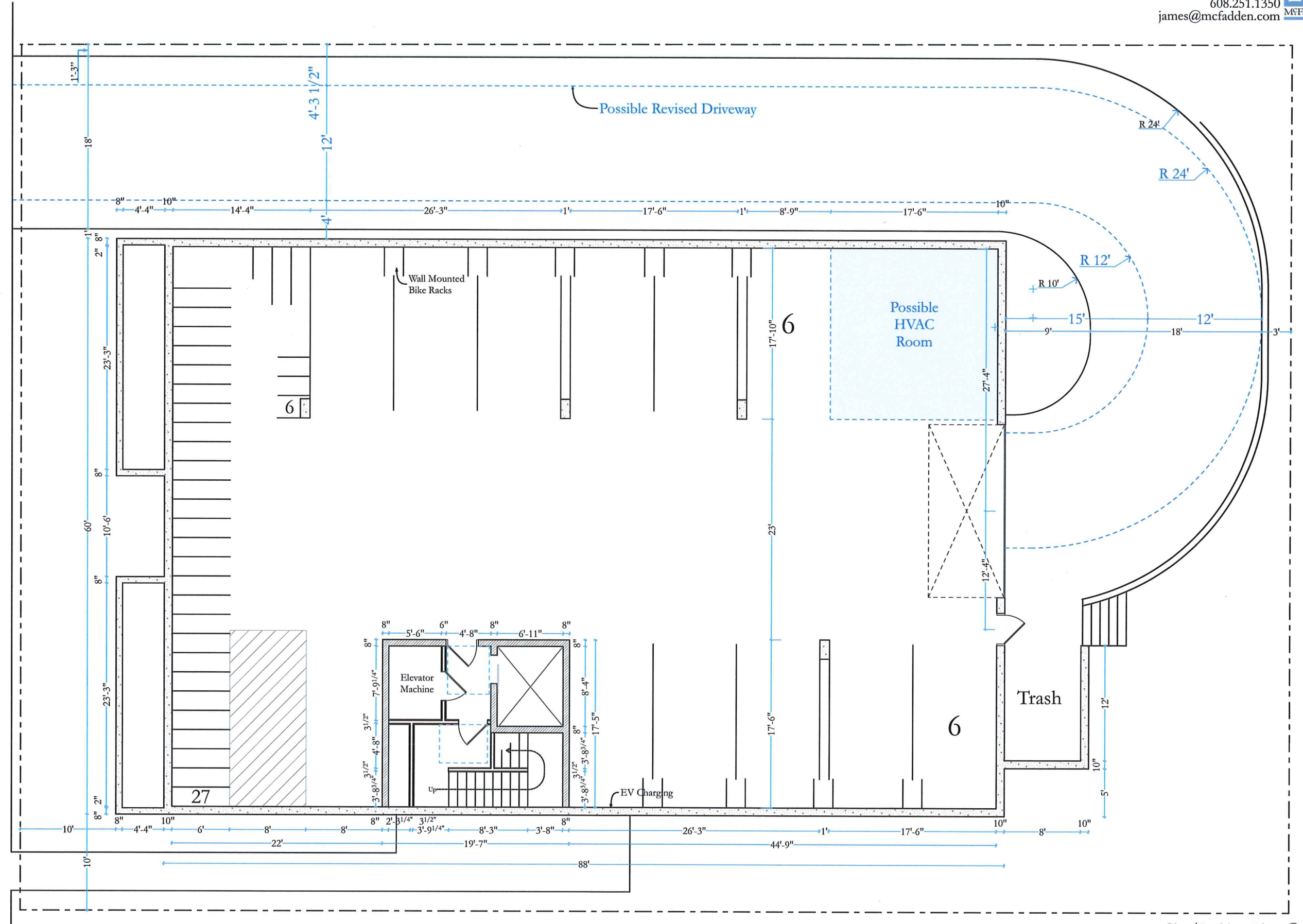
Site/Parking Plan @ 1"-10' 121 North Butler September 20, 2018
