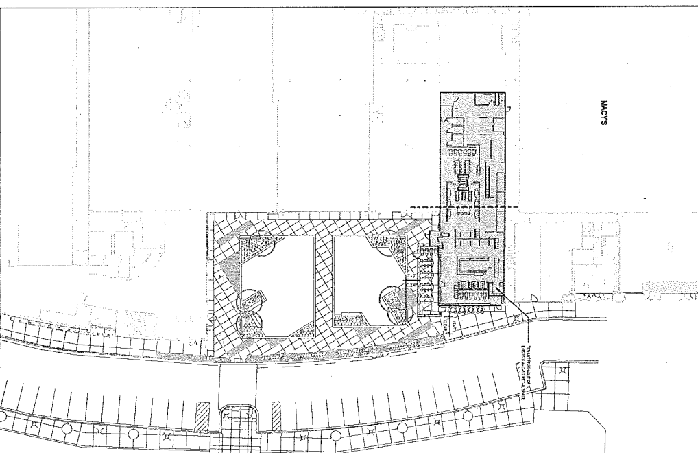
41 BUILDING PLAN / SITE PLAN 1" = 20'-0"
