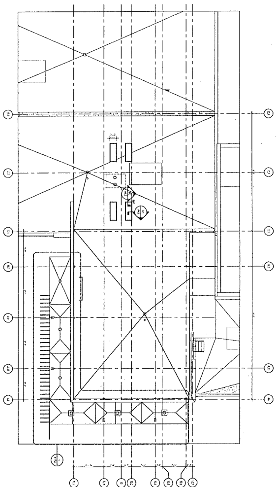
ROOF PLAN 1/8" = 1'-0"
