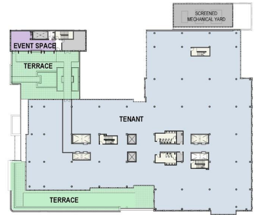
LEVEL 04 PLAN
