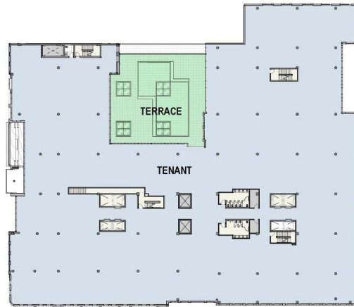
LEVEL 03 PLAN
