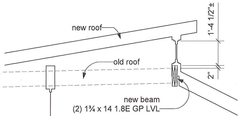
2 Detail - Roof Section 11 Scale: 3/8" = 1'-0"
