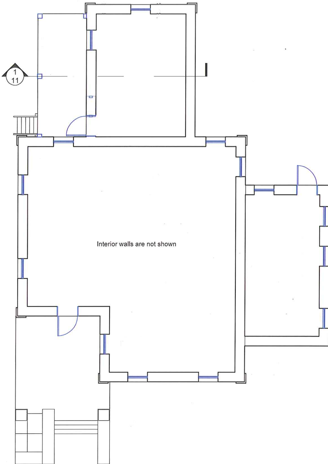
1 Floor Plan-1 2 Scale: 1/8" = 1'-0"
