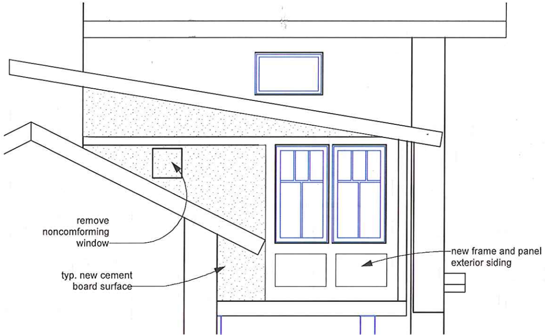
1 South Elevation 8 Scale: 1/4" = 1'-0"
