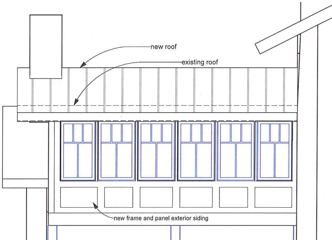
2 East Elevation Detail 8 Scale: 1/4" = 1'-0"
