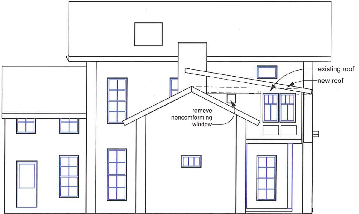
2 South Elevation 6 Scale: 1:100
