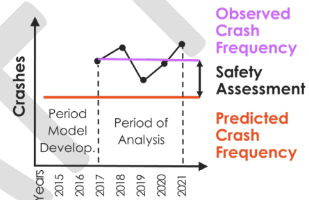
Fig. 4 Safety assessment
