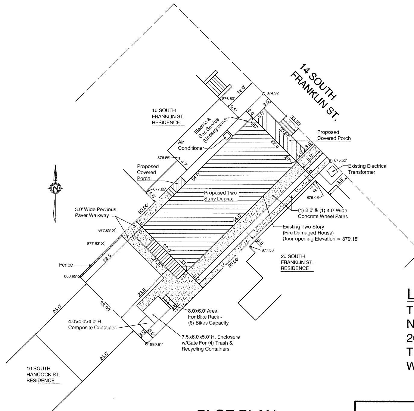
PLOT PLAN Scale: 1" = 20'-0"
