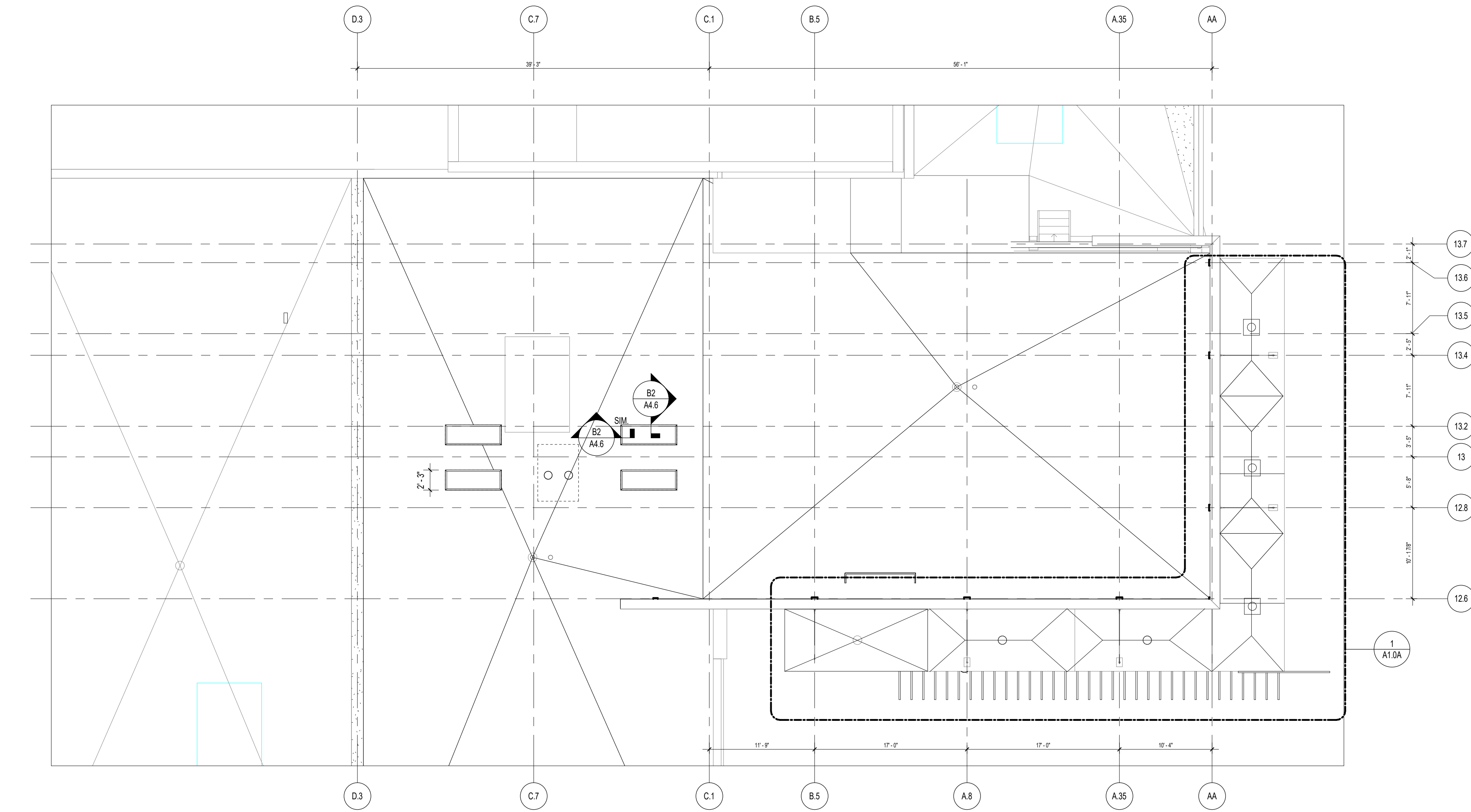
ROOF PLAN 1/8" = 1'-0"
