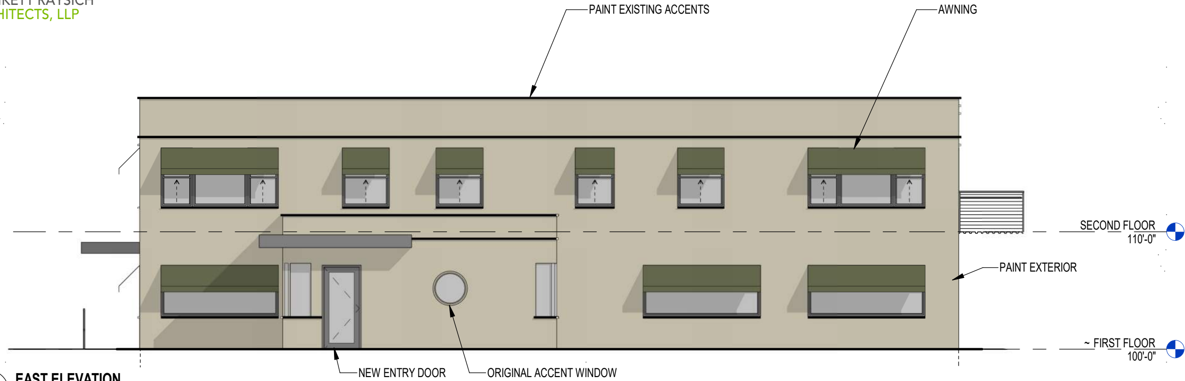
1 EAST ELEVATION 1/8" = 1'-0"
