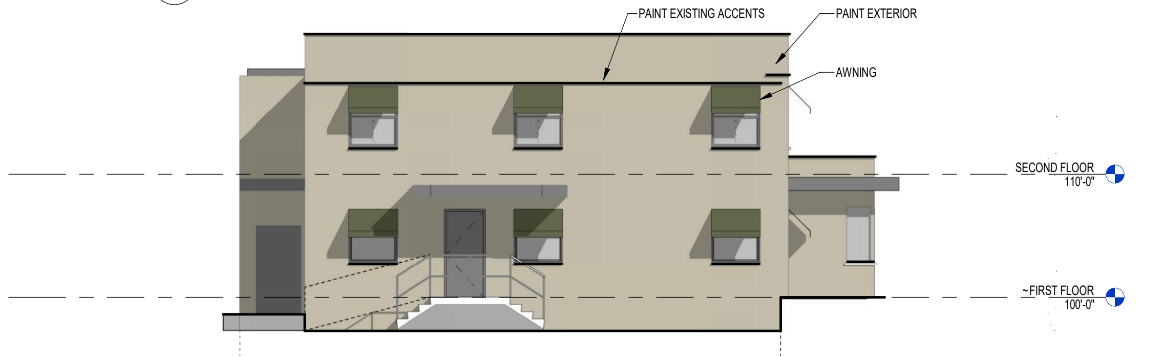
4 SOUTH ELEVATION 1/8" = 1'-0"
