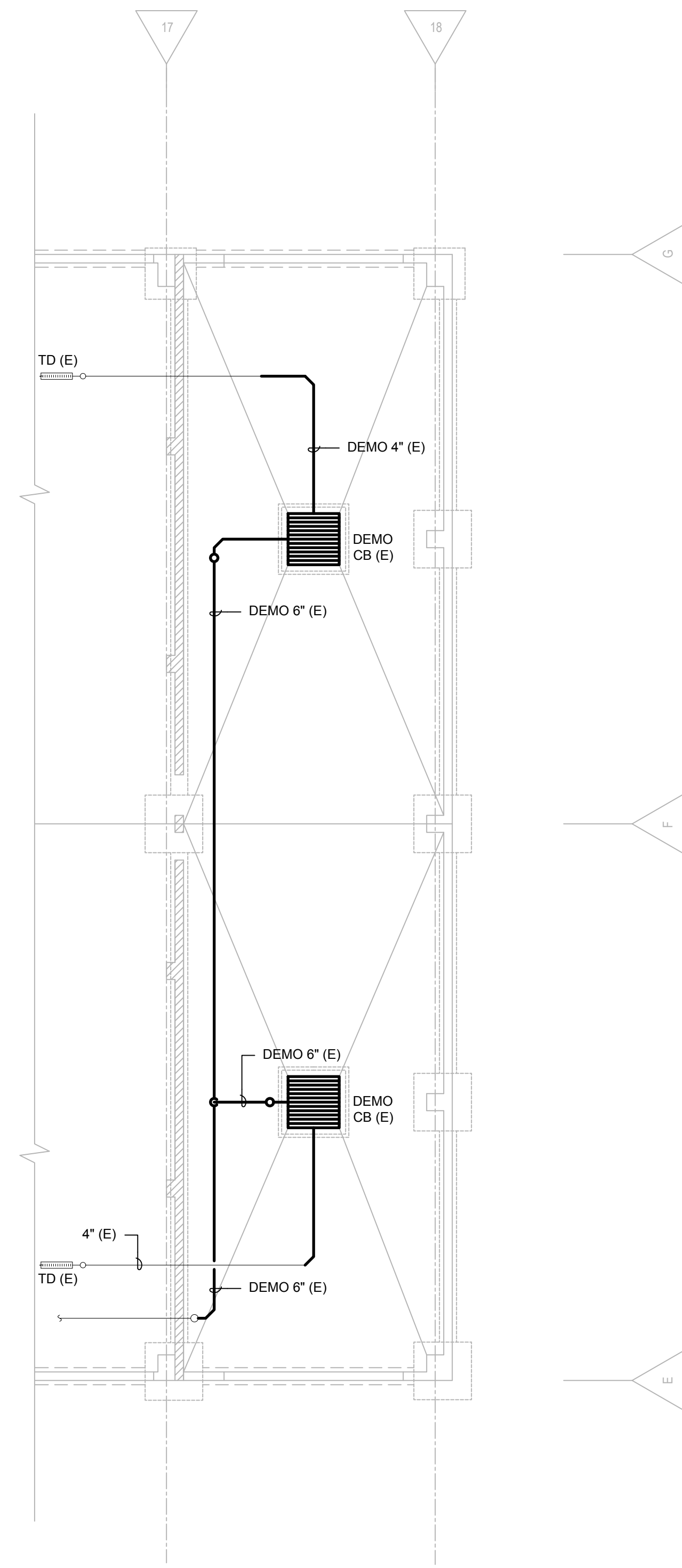
1 DEMOLITION UNDERFLOOR PLAN - PLUMBING P200 SCALE: 1/8"=1'-0"
