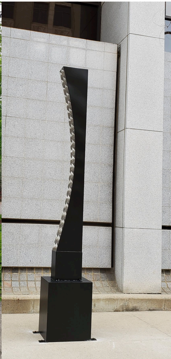
Arc II , painted & stainless steel, 180 lbs, 120”H x 16”W x 19”D Footprint: 24” x 34” bolt to concrete or spot weld to steel
