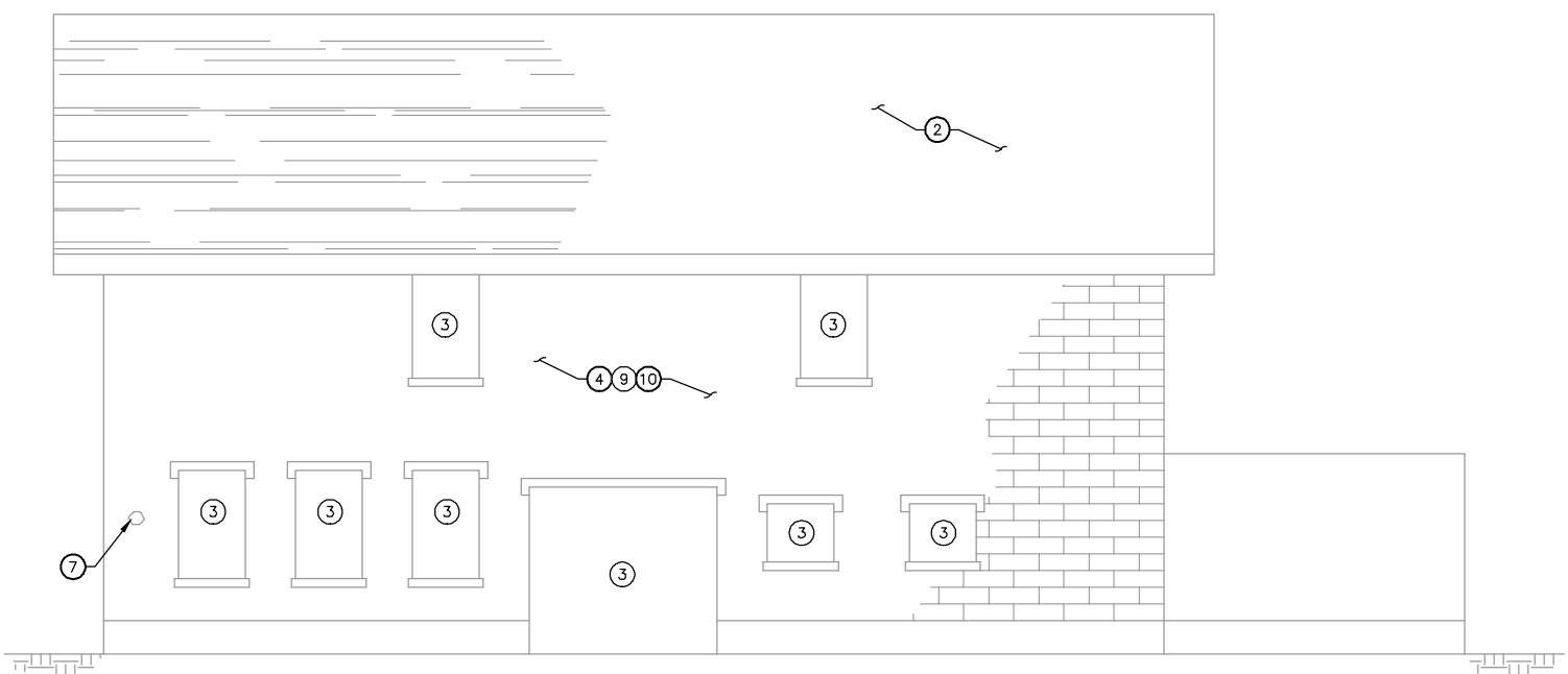
EAST ELEVATION 0 2' 4' 8' 16'
