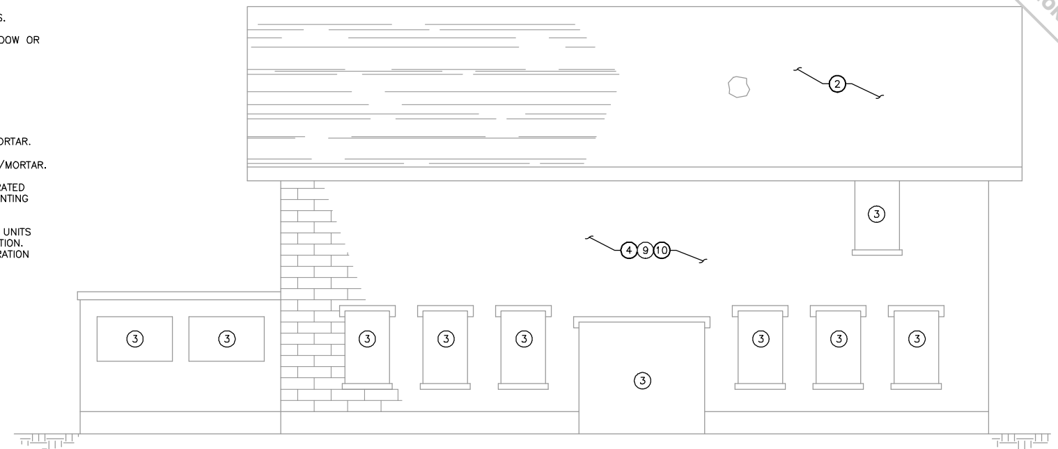
WEST ELEVATION 0 2' 4' 8' 16'
