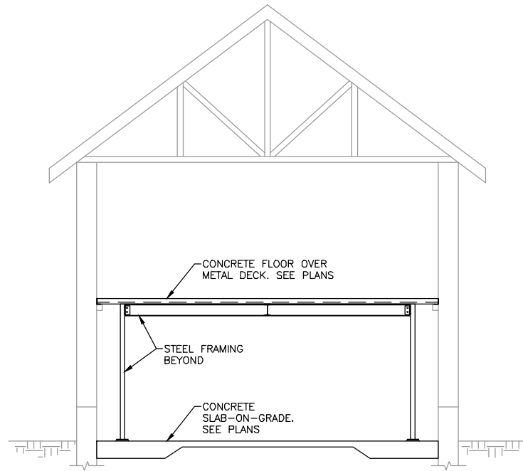
SECTION 1 AS3.1
