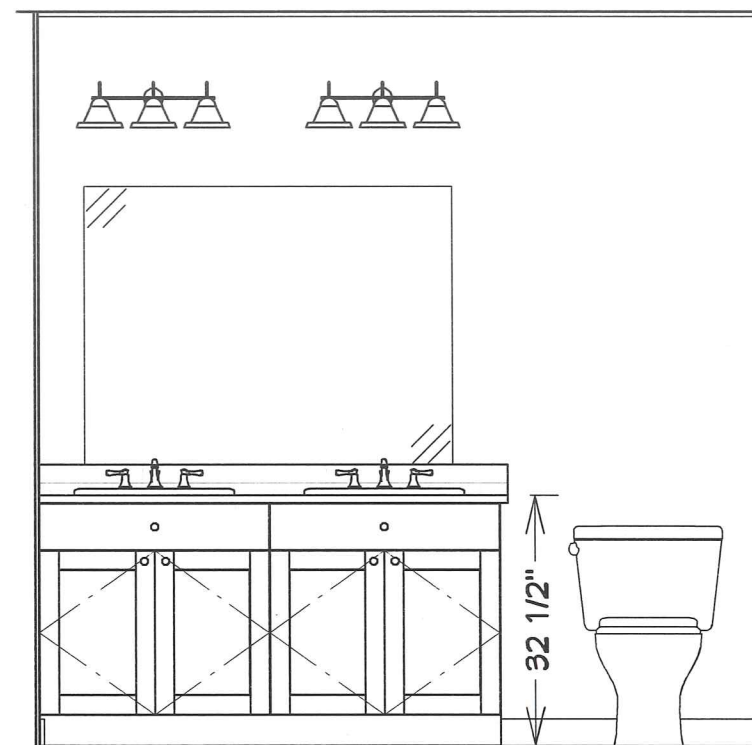
MASTER BATH (VANITY ELEVATION)
