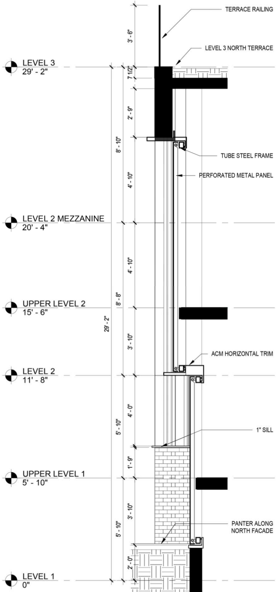
WALL SECTION
