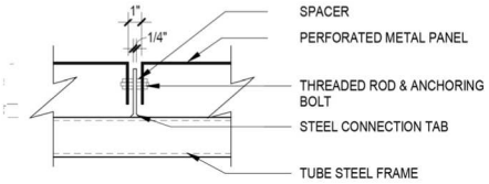
PANEL PLAN DETAIL
