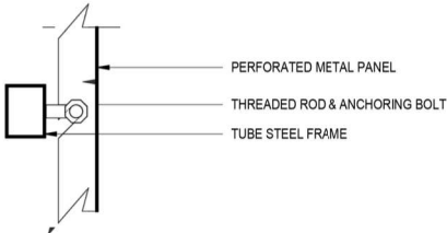
PANEL SECTION DETAIL
