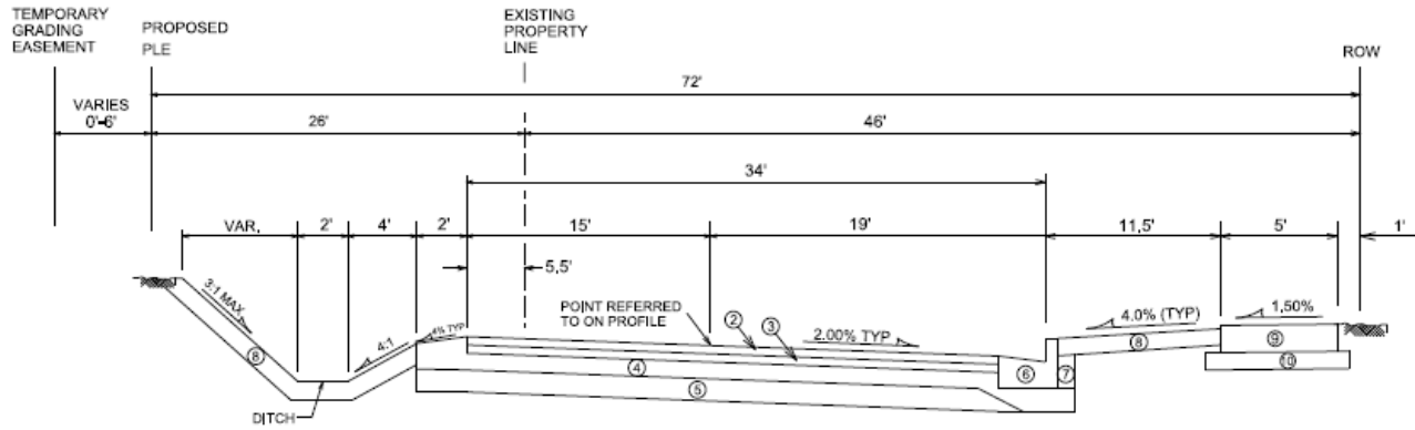
TYPICAL FINISHED SECTION DILORETO AVENUE STATION 15+50 to STATION 19+00 NOT TO SCALE
