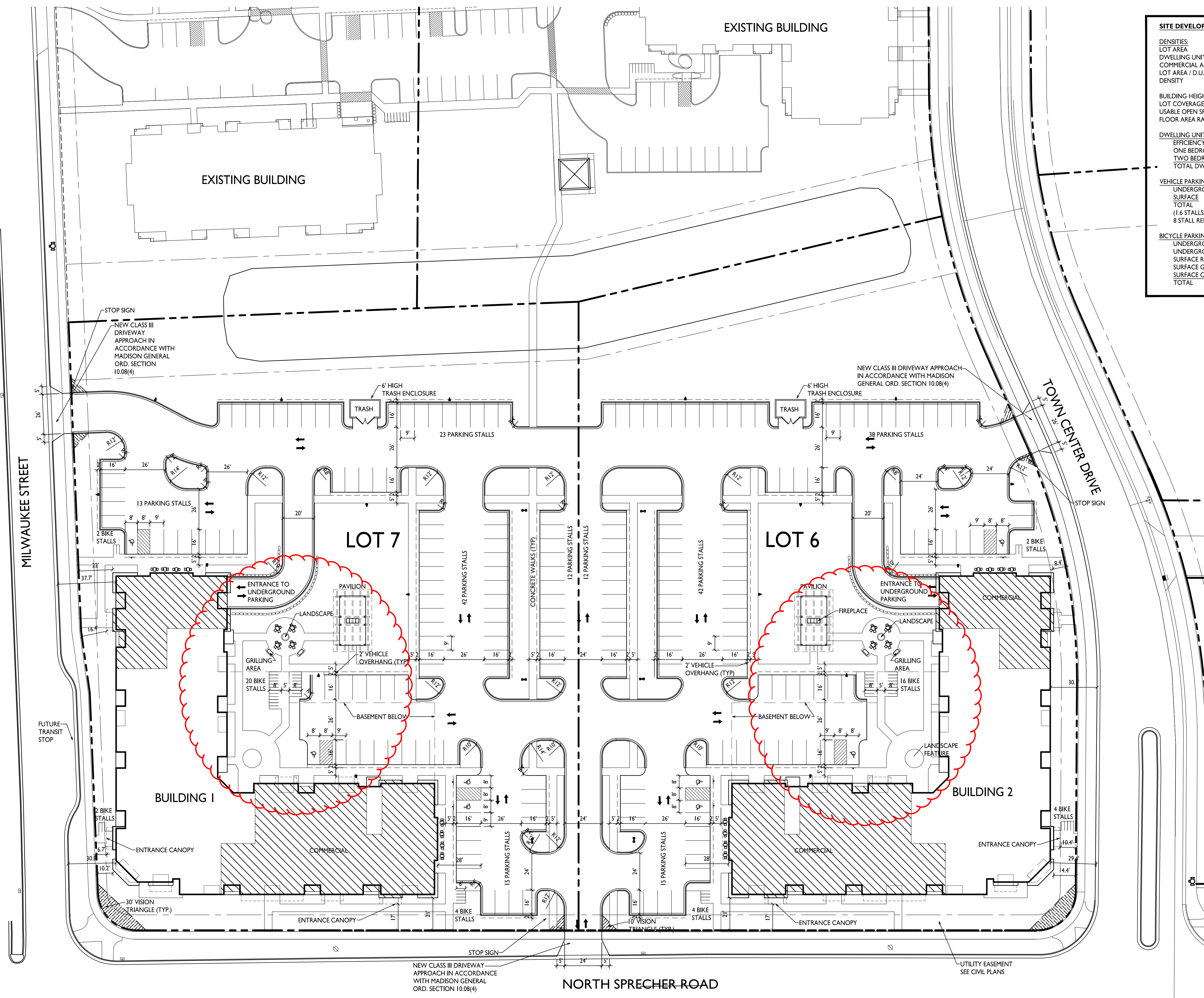
SITE PLAN C-1.1 1" = 30'-0"
