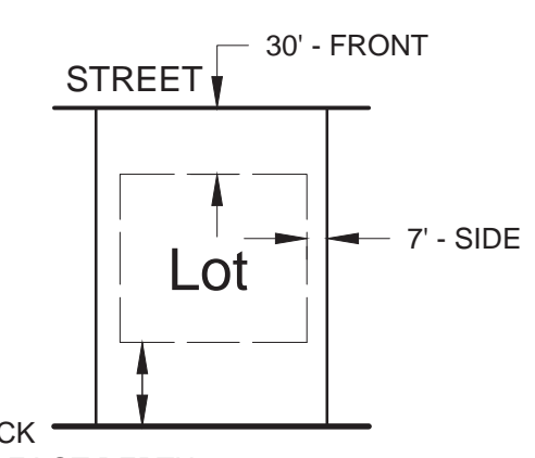
TYPICAL-BUILDING SETBACK TWO STORY
