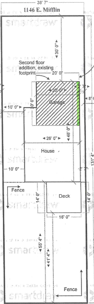
1146 E. Mifflin Site Plan 15/16" = 20'
