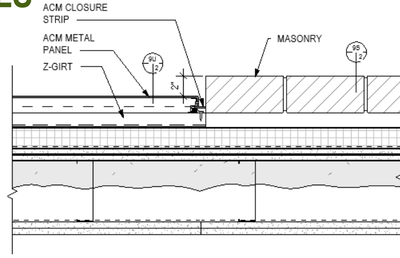
7 PLAN SECTION WALL TRANSITION @ ACM AND MASONRY 1 1/2" = 1'-0"
