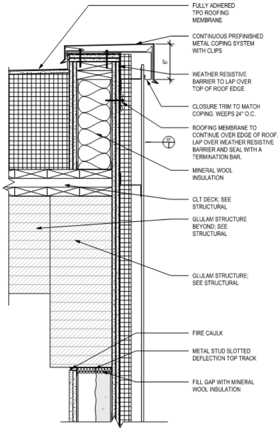
1 ROOF EDGE DETAIL AT METAL PANEL 1 1/2" = 1'-0"
