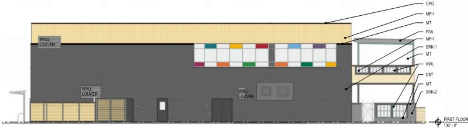
4 NORTH ELEVATION 3/32" = 1'-0"
