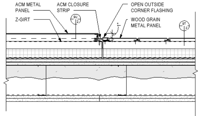
6 PLAN SECTION WALL TRANSITION @ ACM PANEL AND METAL 1 1/2" = 1'-0"
