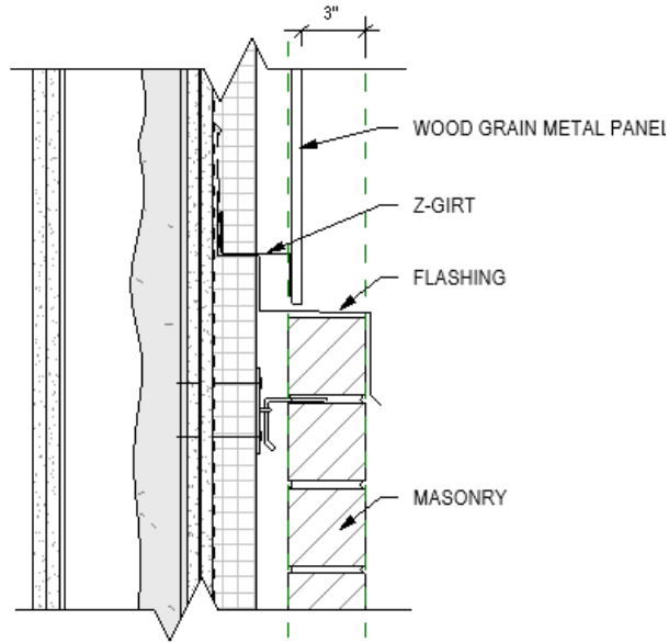
9 METAL PANEL TO BRICK TRANSITION 1 1/2" = 1'-0"
