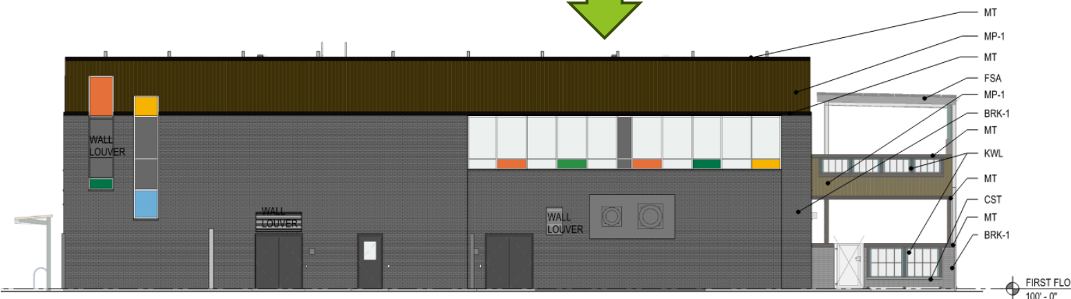
4 NORTH ELEVATION 3/32" = 1'-0"
