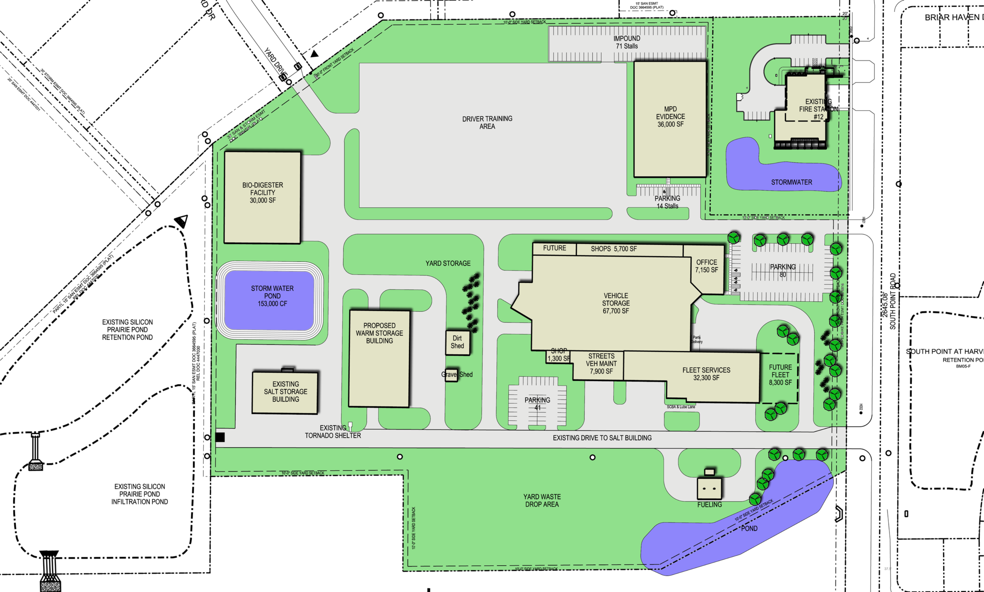
NORTH MASTER SITE PLAN SCALE: 1"=60'-0"
