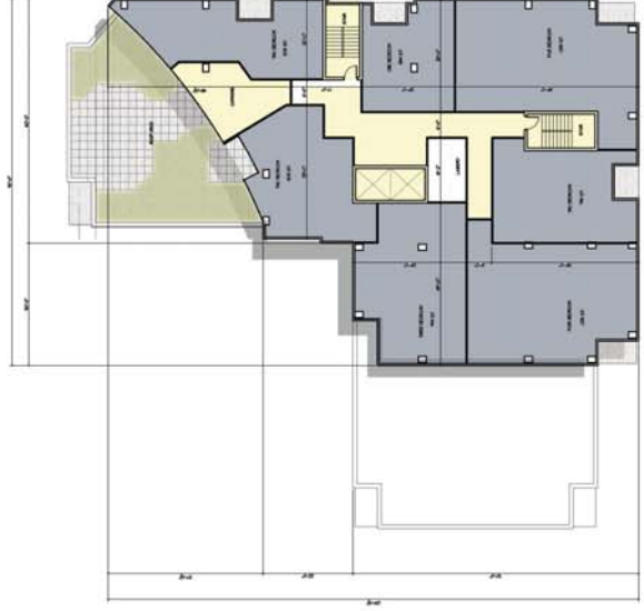
Typical Fifth-Eighth Floor Plan
