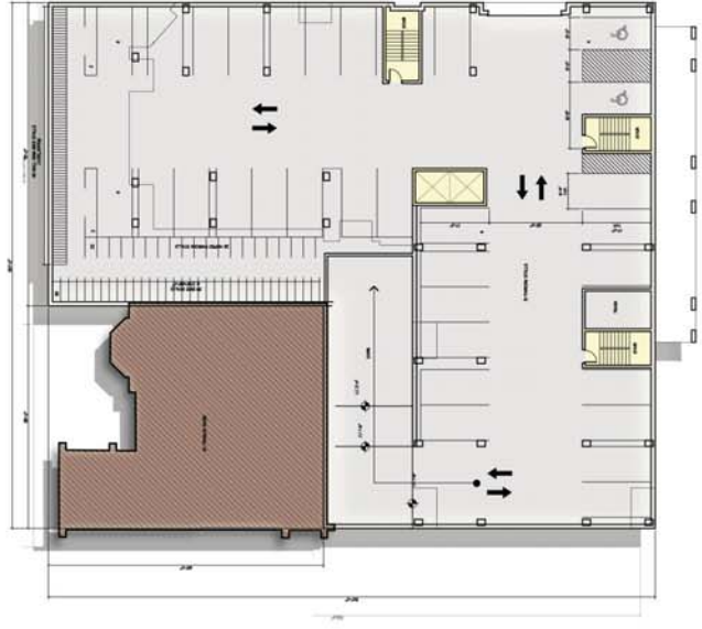
Typical Basement Plan
