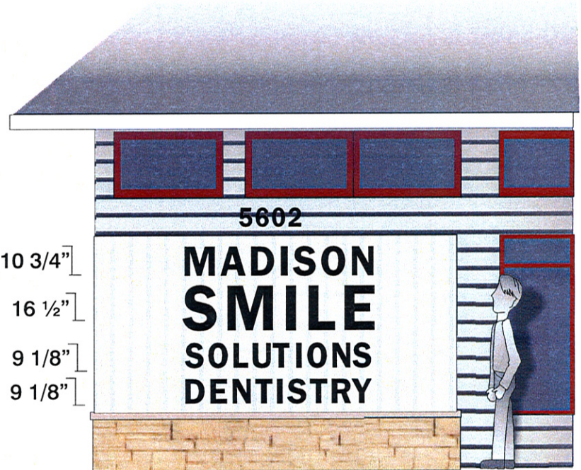
South Elevation
