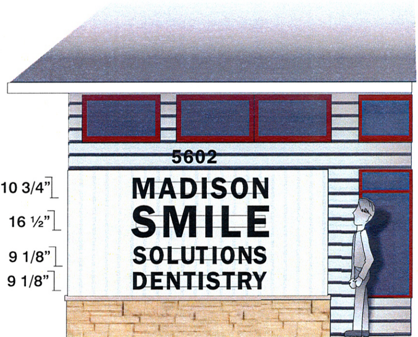
South Elevation
