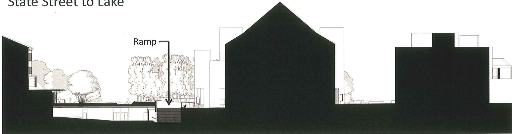
Section Loading Dock Ramp A-A'
