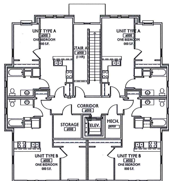
2 SECOND FLOOR PLAN A-1.1 1/8"=1'-0"
