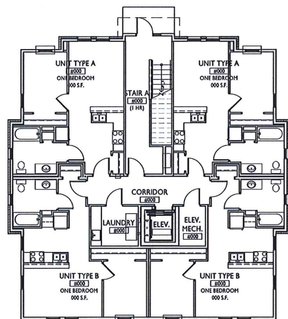
1 FIRST FLOOR PLAN A-1.1 1/8"=1'-0"
