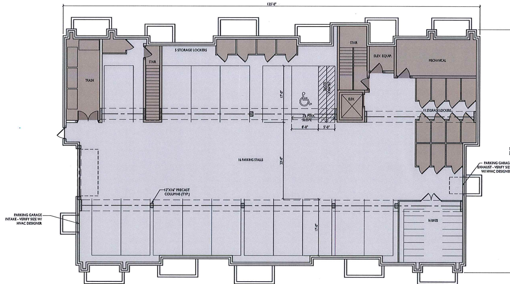
Basement Plan
