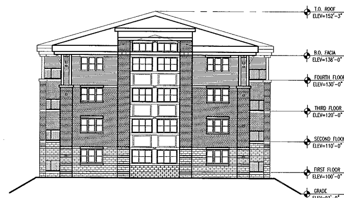
4 EAST ELEVATION (YELLOWSTONE DRIVE) 0 8' 16' 32'
