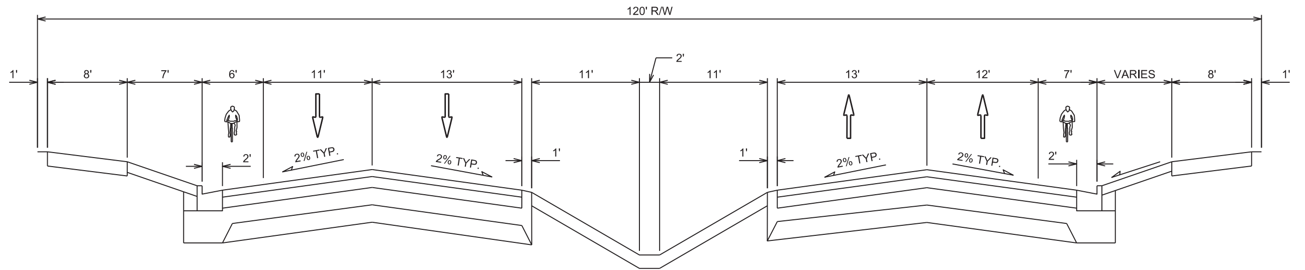
ULTIMATE FINISHED SECTION HOEPKER ROAD
