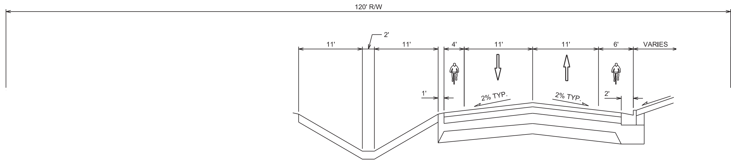
TYPICAL FINISHED SECTION HOEPKER ROAD
