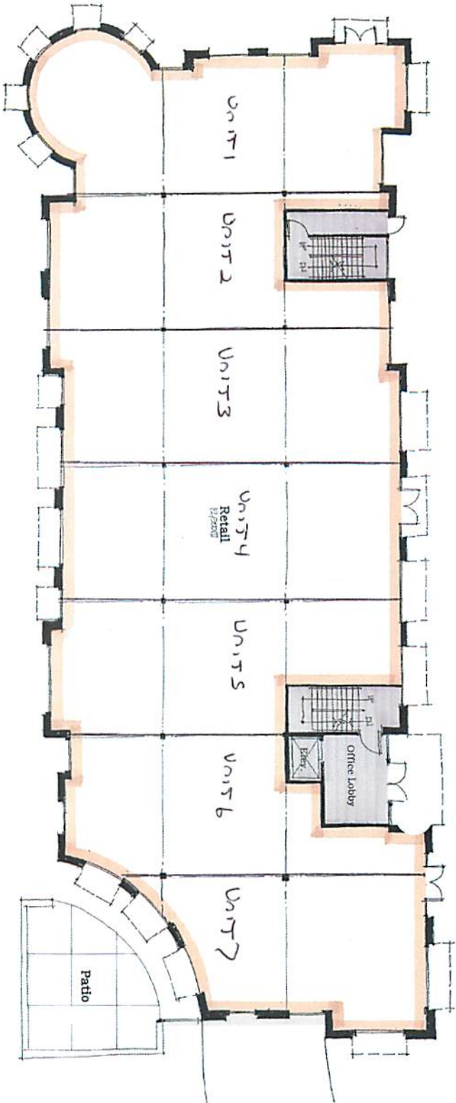
Building A First Floor Plan
