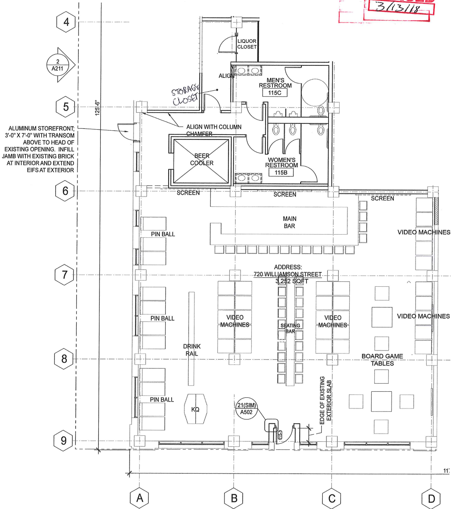
1 BUILDING-(B) GRADE FLOOR PLAN
