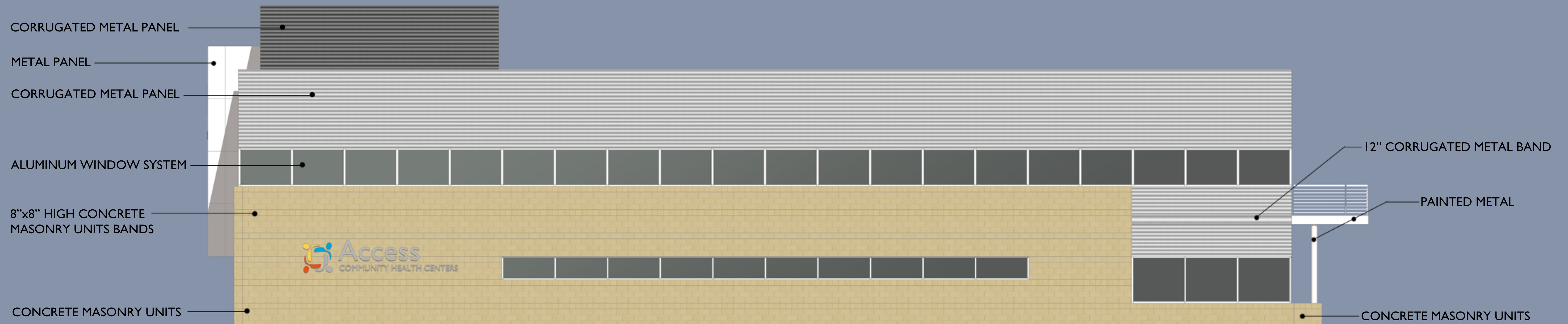
NORTH ELEVATION
