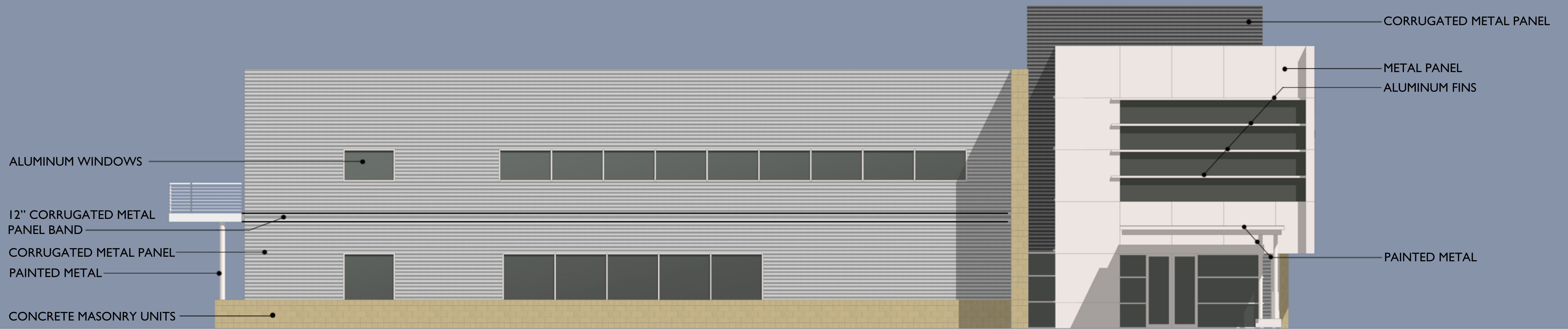
SOUTH ELEVATION
