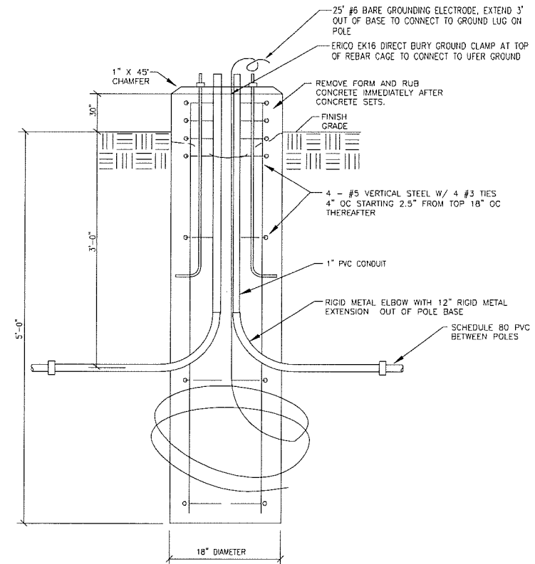
2 POLE BASE DETAIL SCALE: NOT TO SCALE
