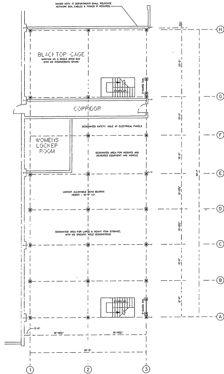
CONCEPTUAL MAIN FLOOR PLAN
