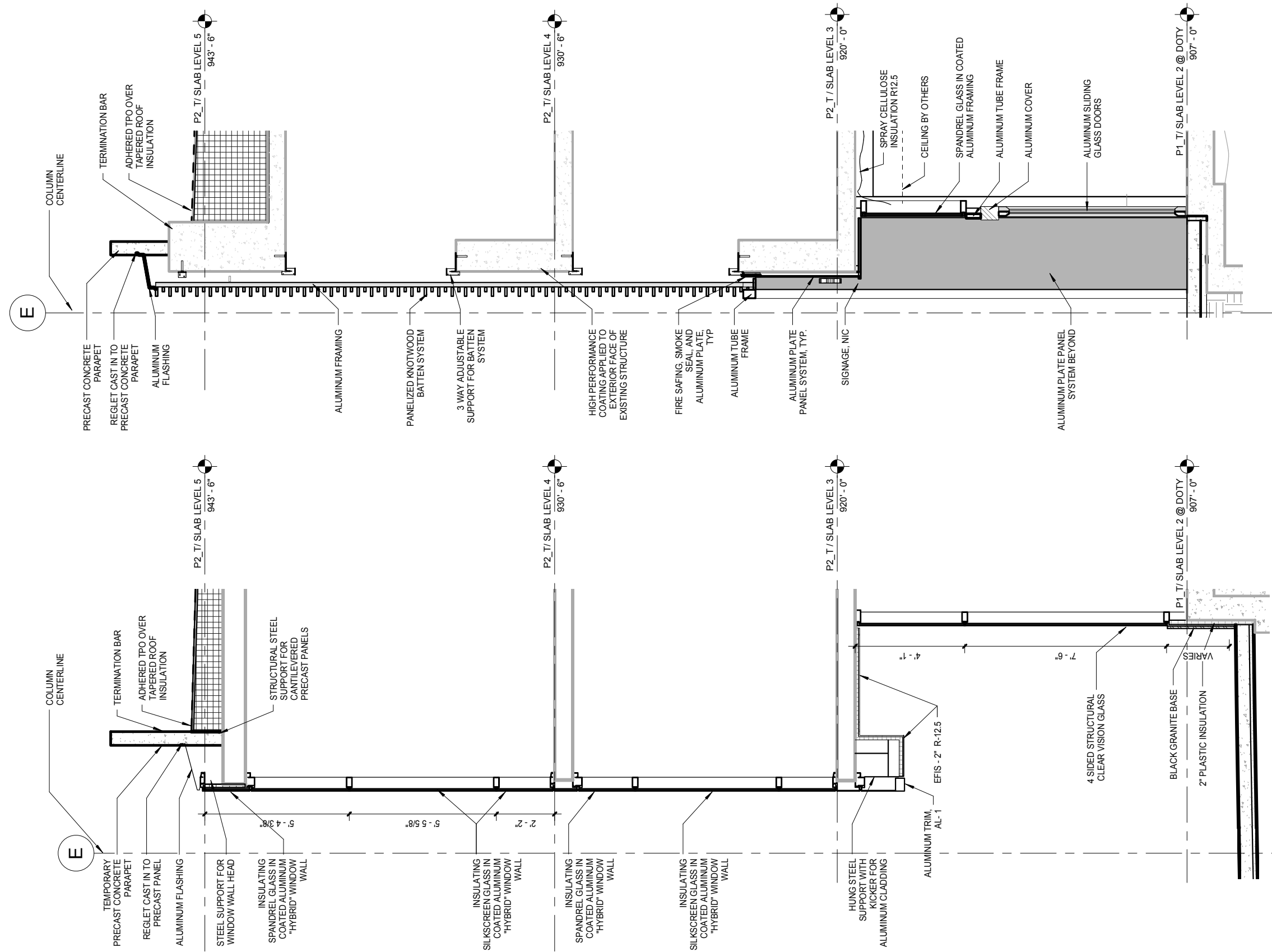
WALL SECTION AT TEMPORARY CAP ON PINCKNEY STREET
