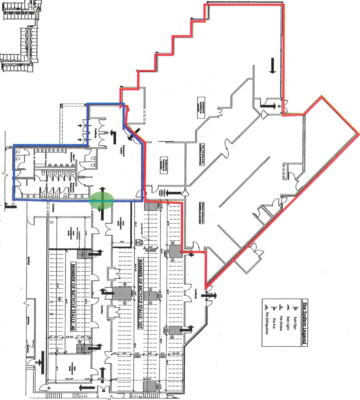
1 Restaurant Area - Partial Floor Plan SCALE: 1/8" = 1'-0" (24"x36" - Full size) 1/16" = 1'-0" (12"x18" - Half size)
