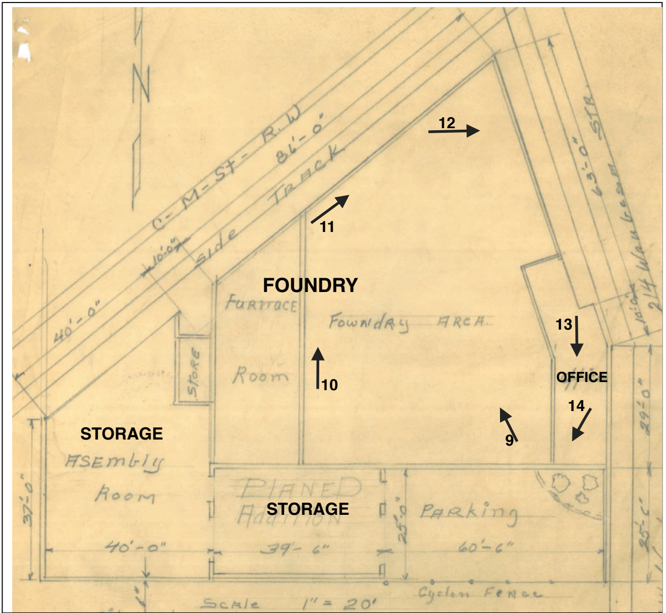
Figure 3. Madison Brass Works Madison, Dane County, Wisconsin Plan with Photo Key
