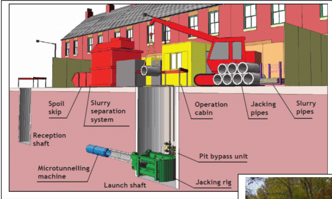
Micro-Tunneling Schematic: Only the launching/receiving pit areas are excavated.
