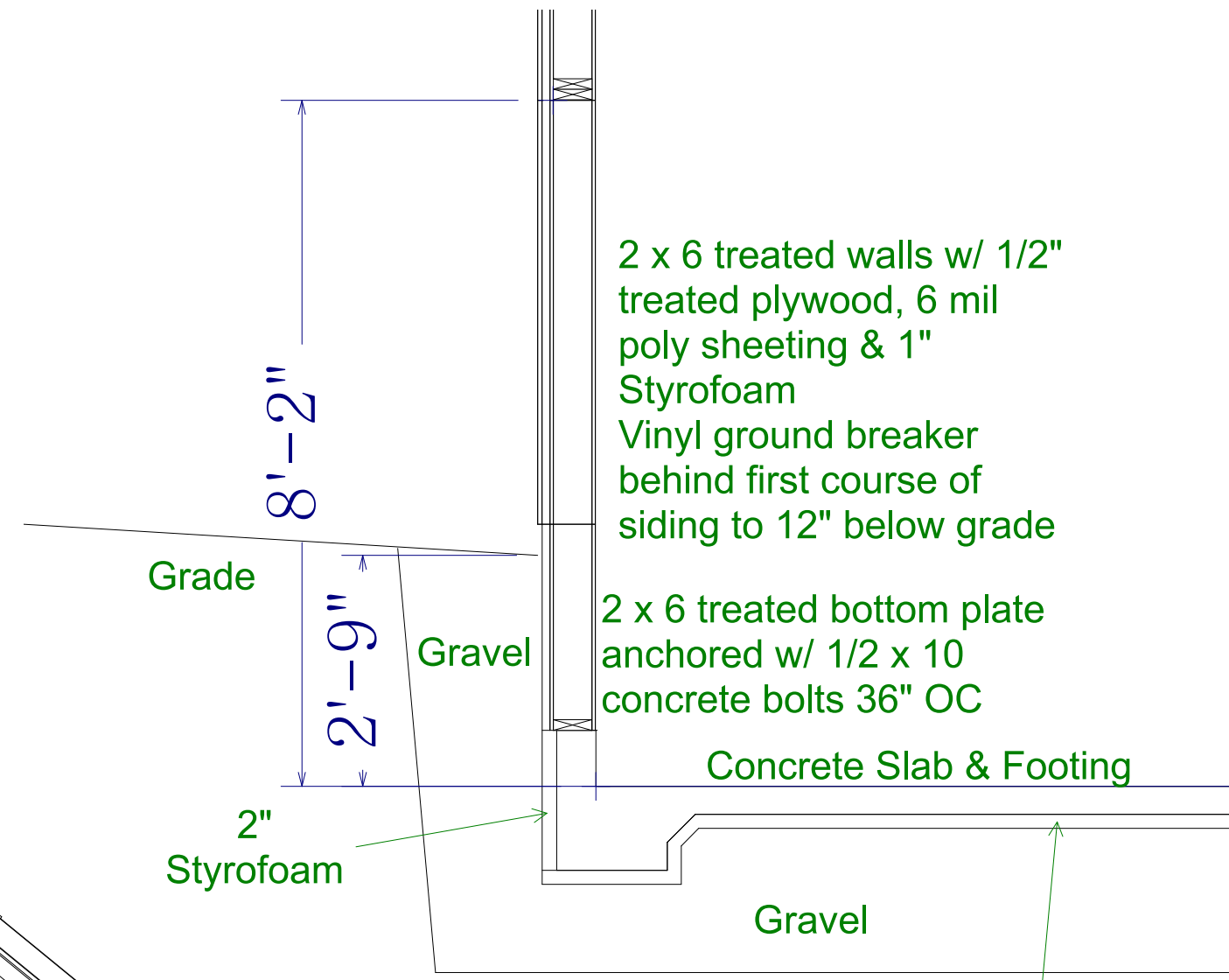
Wall/floor section 1/2" = 1'0"
