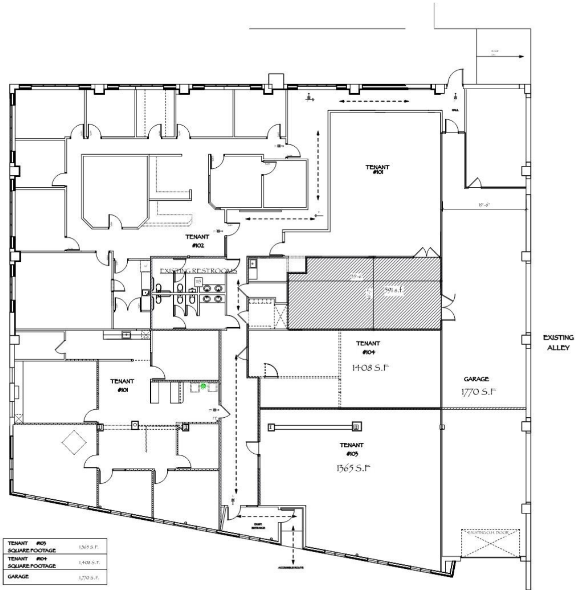
1 FIRST FLOOR PLAN Scale: 1/8" = 1'-0"
