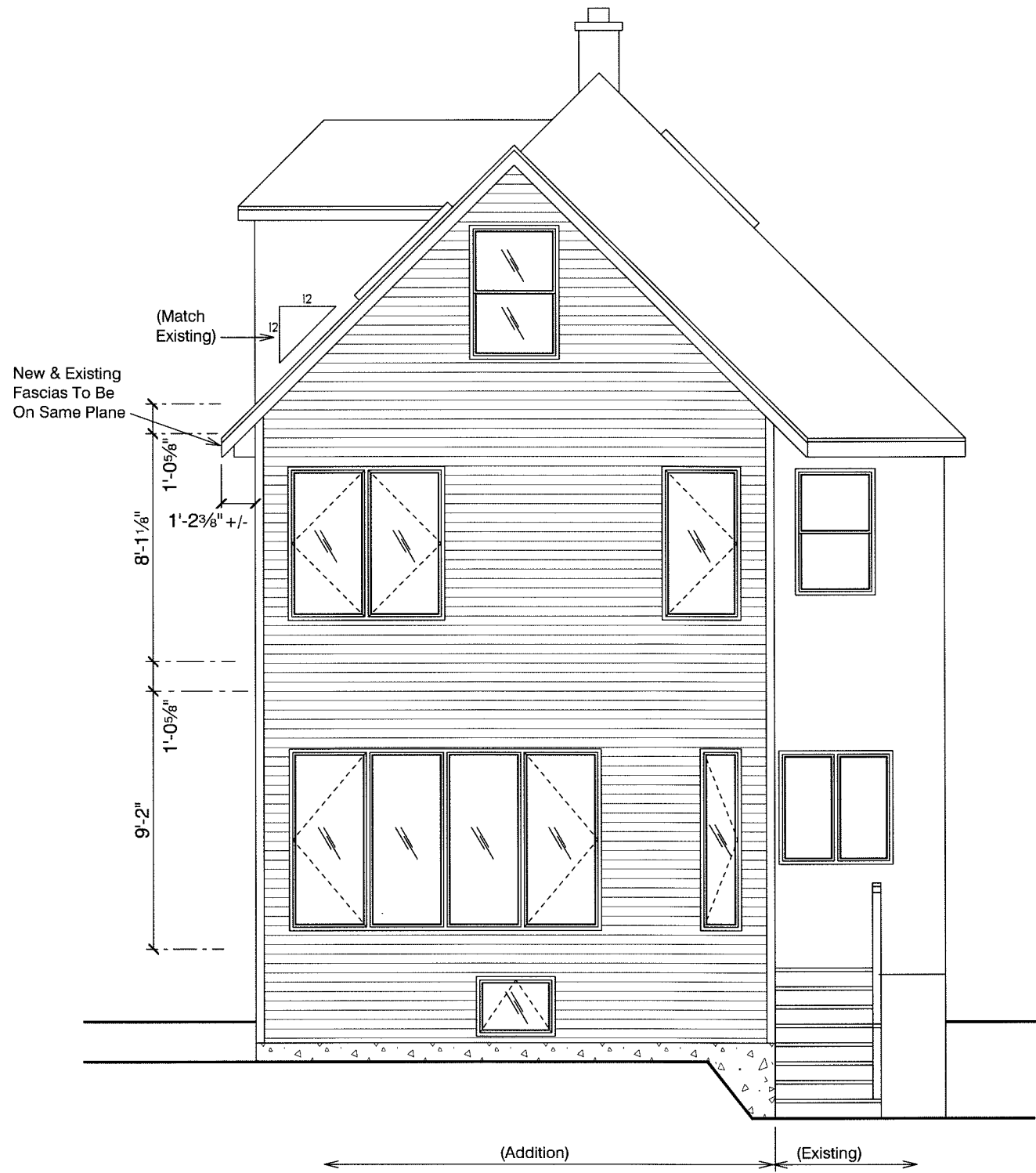
REAR ELEVATION
