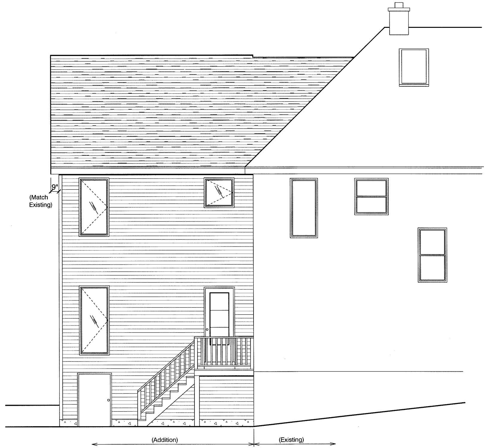
LEFT ELEVATION
