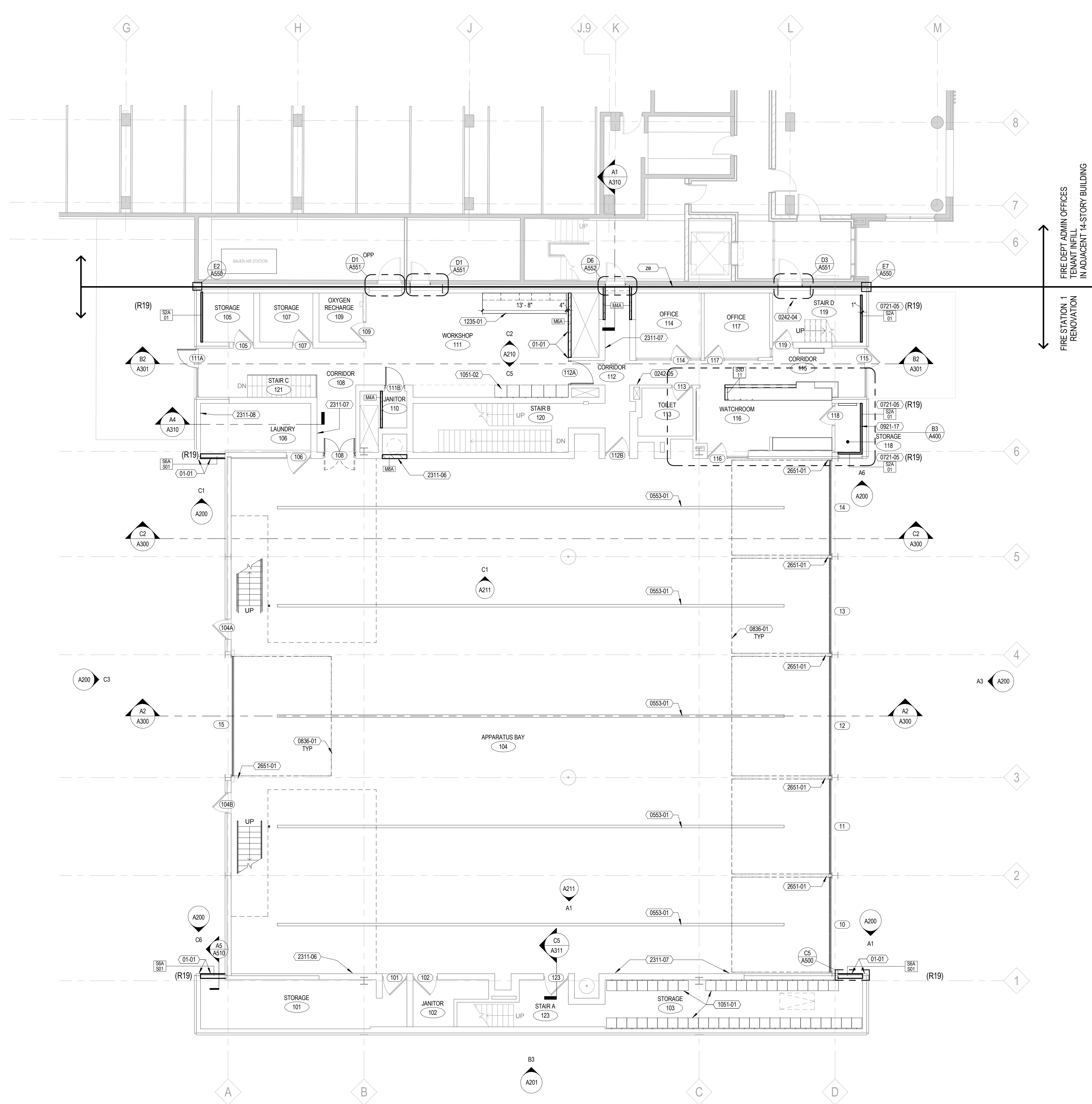
A2 STATION 1 FIRST FLOOR PLAN 1/8" = 1'-0"
