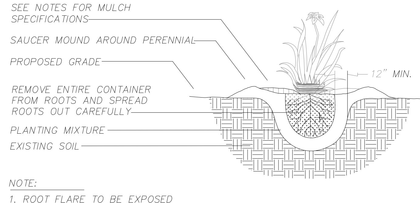
PERENNIAL/ORNAMENTAL GRASS PLANTING DETAIL
