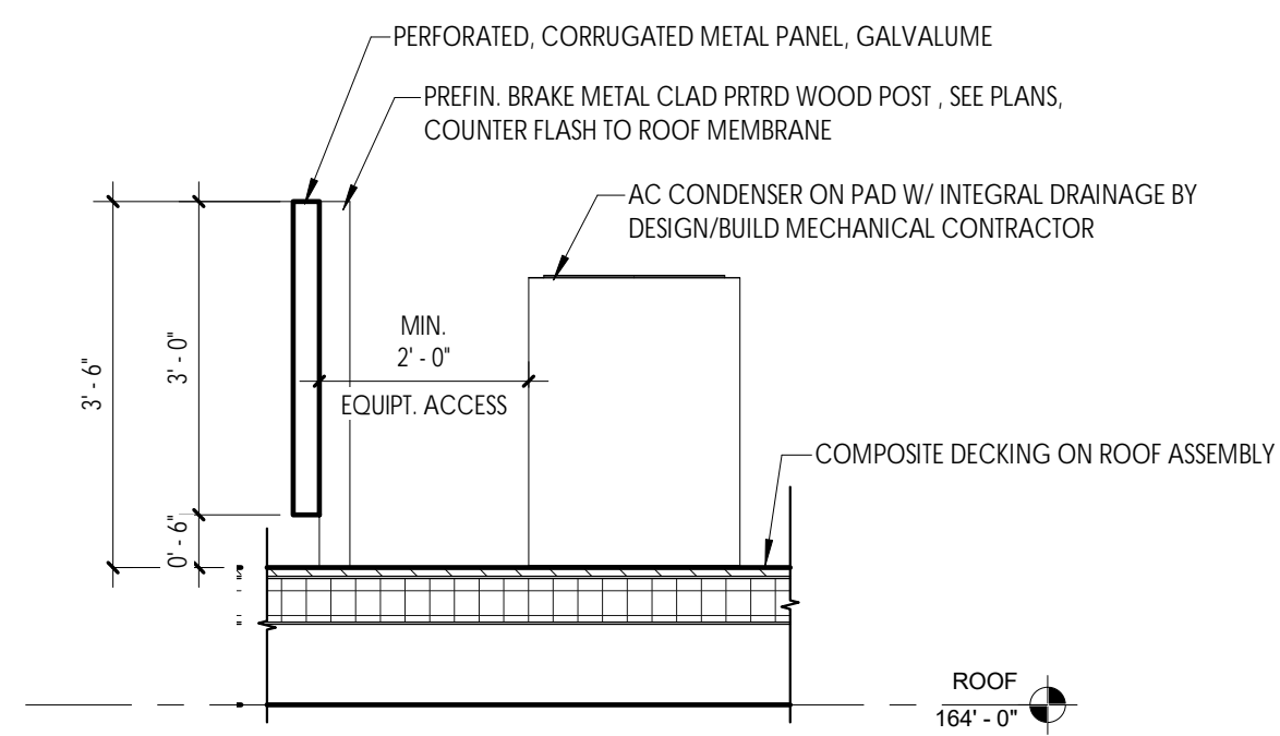
② AC CONDENSER SCREEN DETAIL 1/2" = 1'-0"
