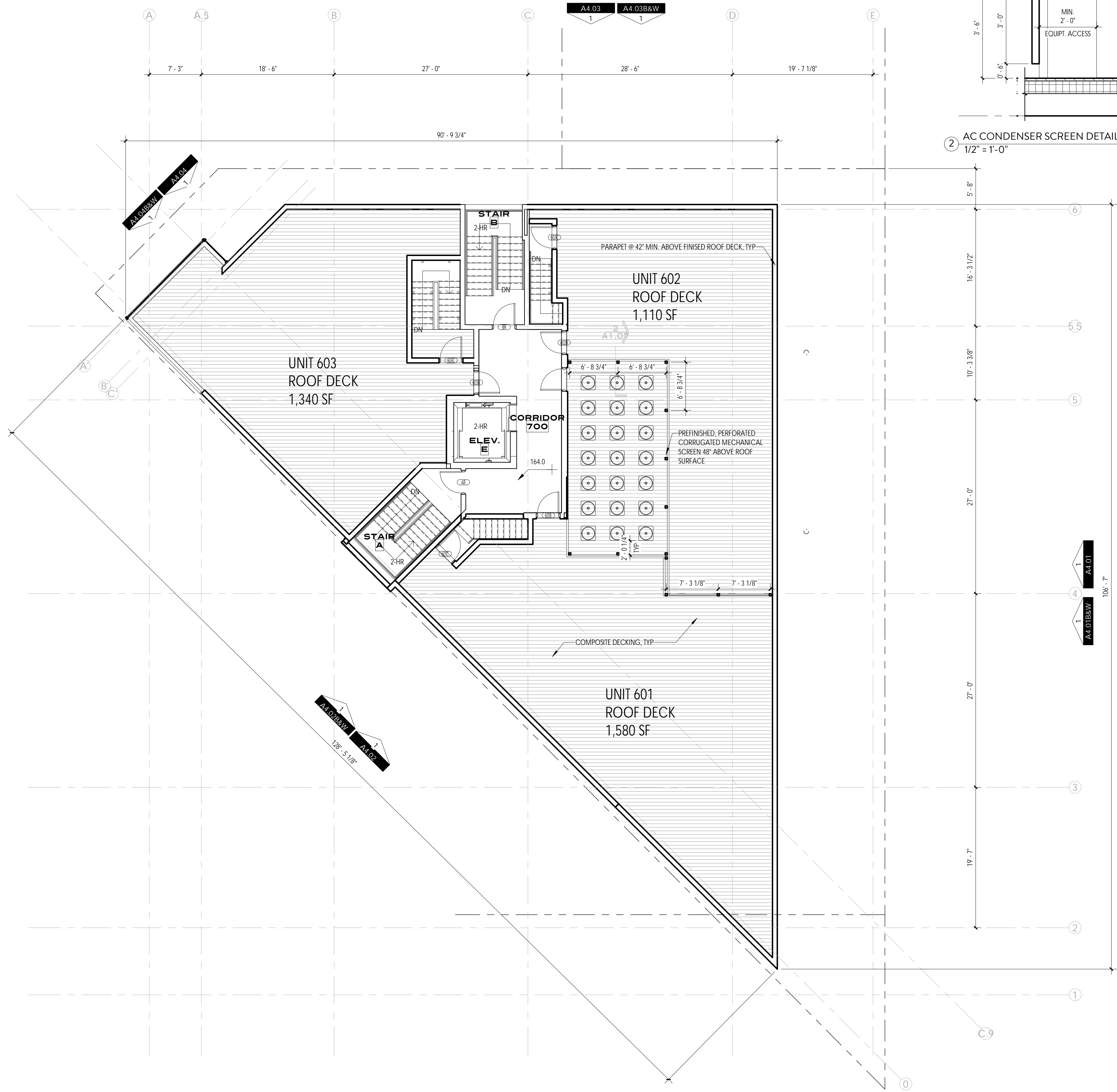
1 ROOF PLAN 1/8" = 1'-0"
