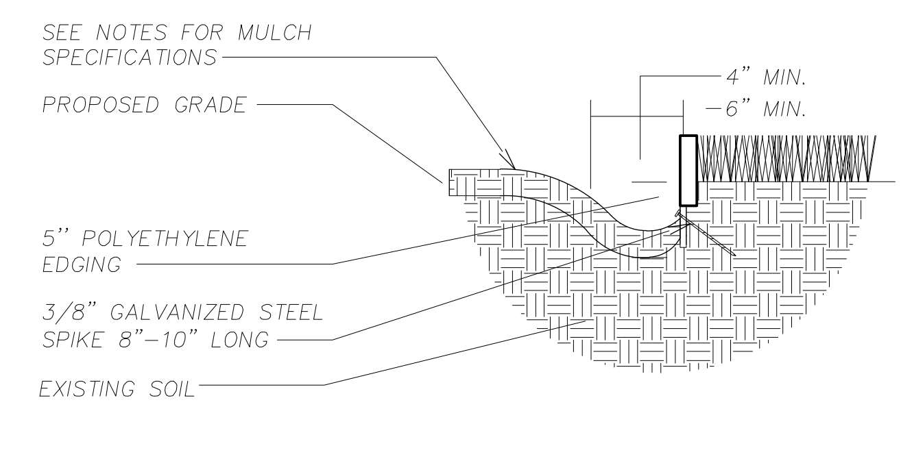
LANDSCAPE EDGING DETAIL
