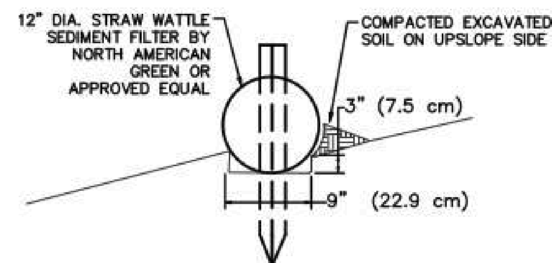
2 SEDIMENT FILTER A6.01 NTS
